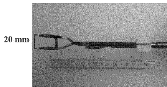
DOUBLE-WOUND COIL WITH LARGE WIDTH
