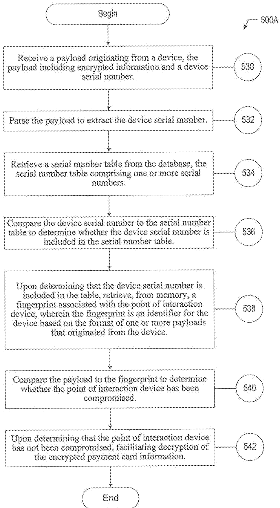
FIG. 5A EXEMPLARY DECRYPTION PROCESS
