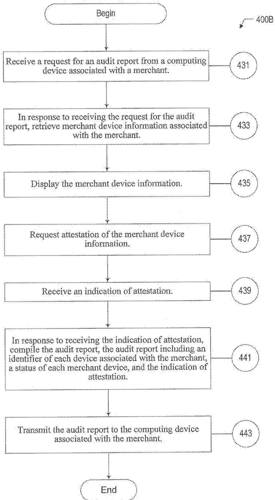
FIG. 4B P2PE REPORT PROCESS
