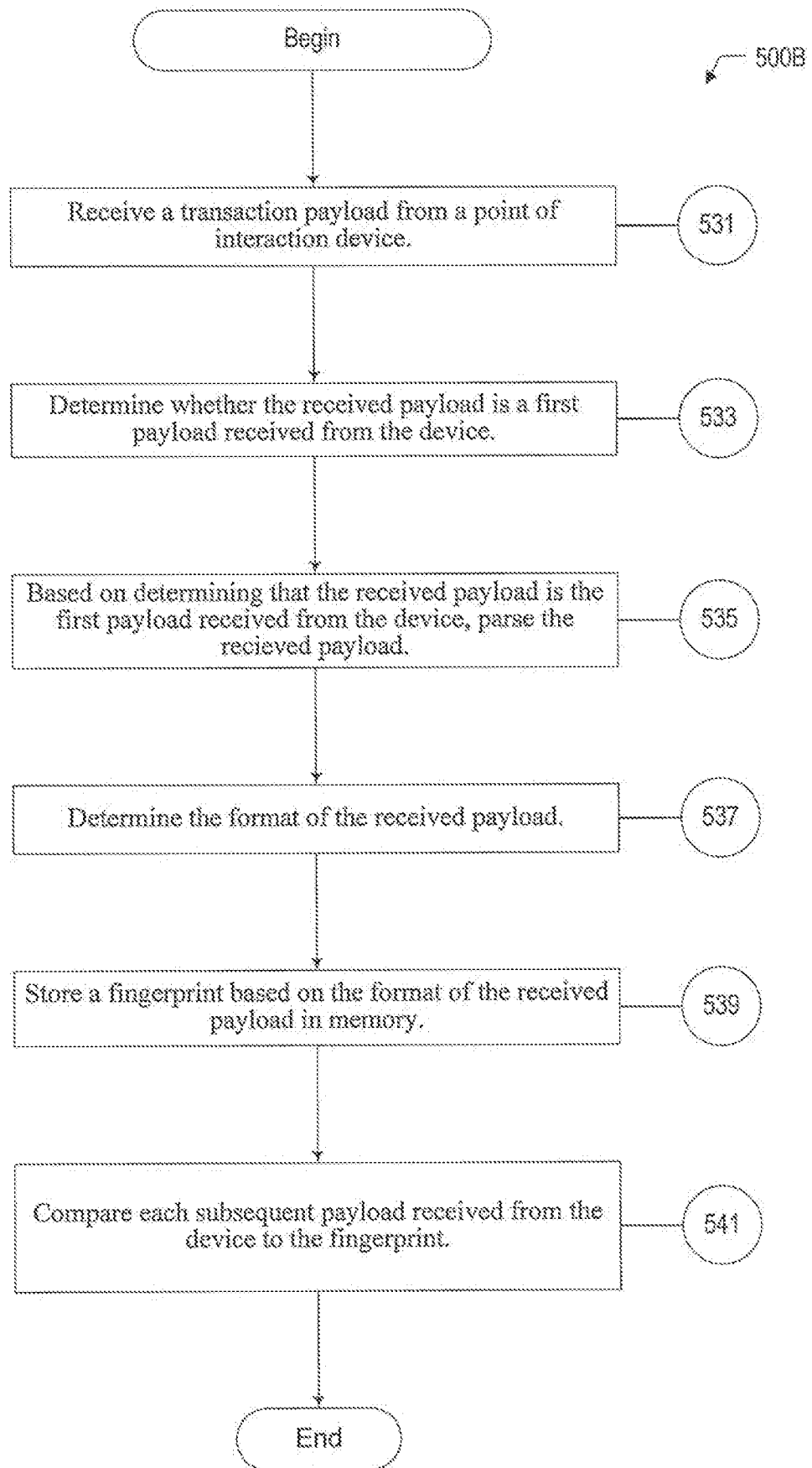
FIG. 5B EXEMPLARY FINGERPRINT PROCESS
