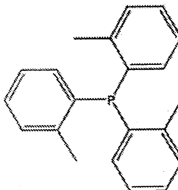
tri-o-tolylphosphine
