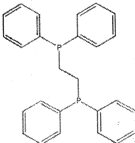
1,2-bis(diphenylphosphino)ethane
