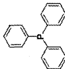
Triphenylphosphine
