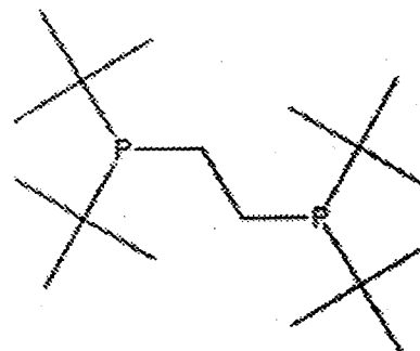
1,2-bis(di-tert-butylphosphino)ethane
