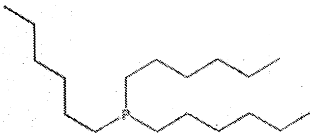
Trihexylphosphine
