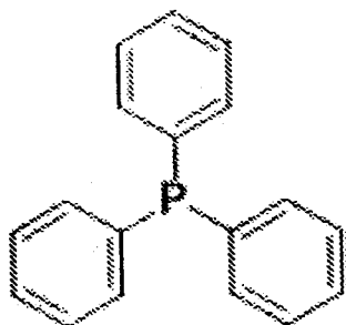
Triphenylphosphine
