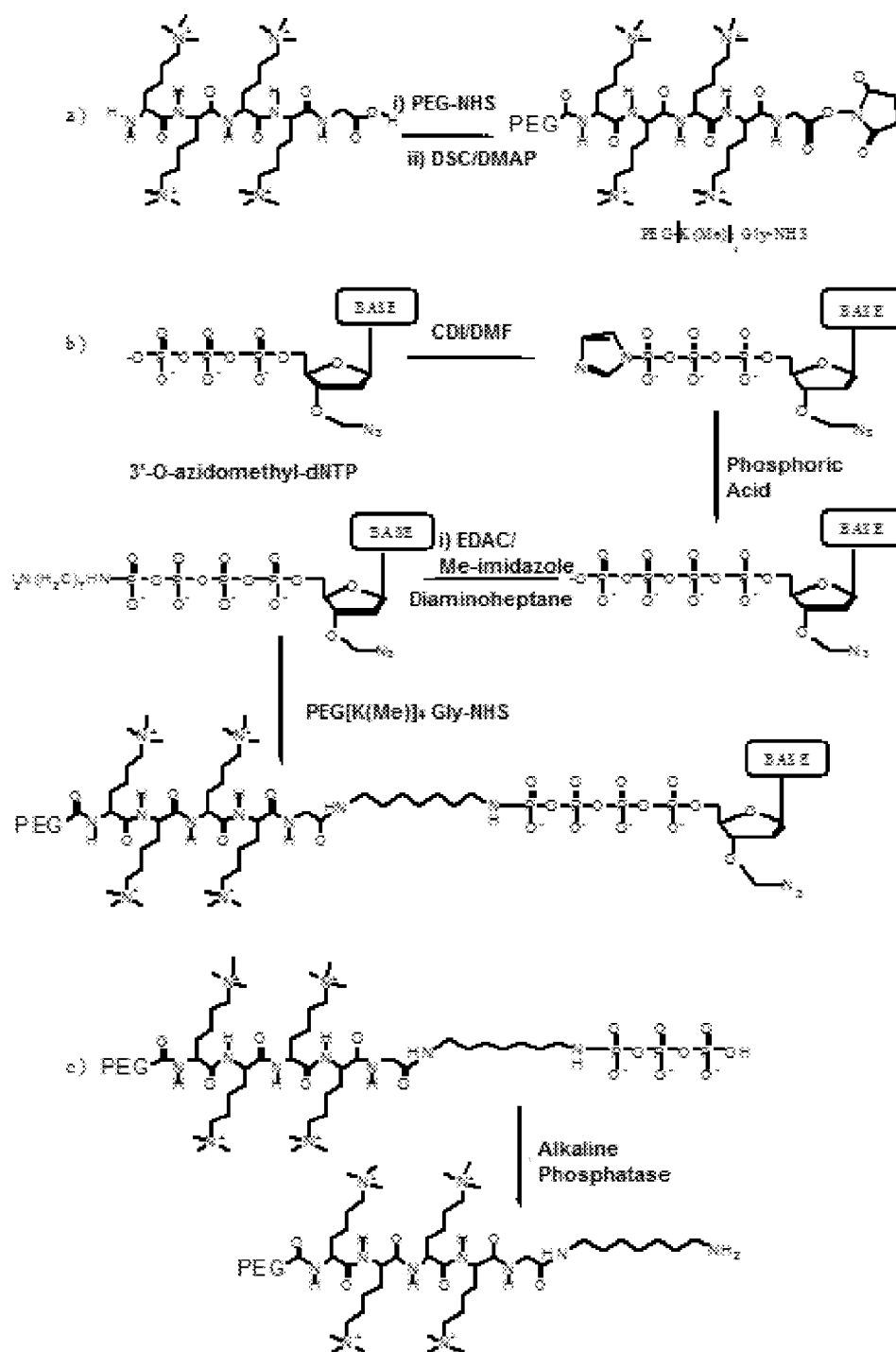
Synthesis of 3'-O-blocked-PEG-nucleotides
