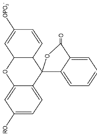
Fluorescein based fluorogenic dyes
