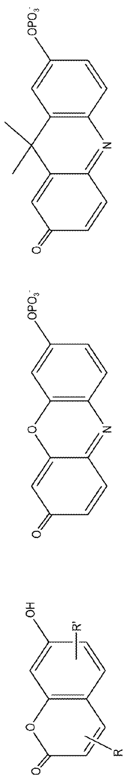
Coumarin based fluorogenic dyes
