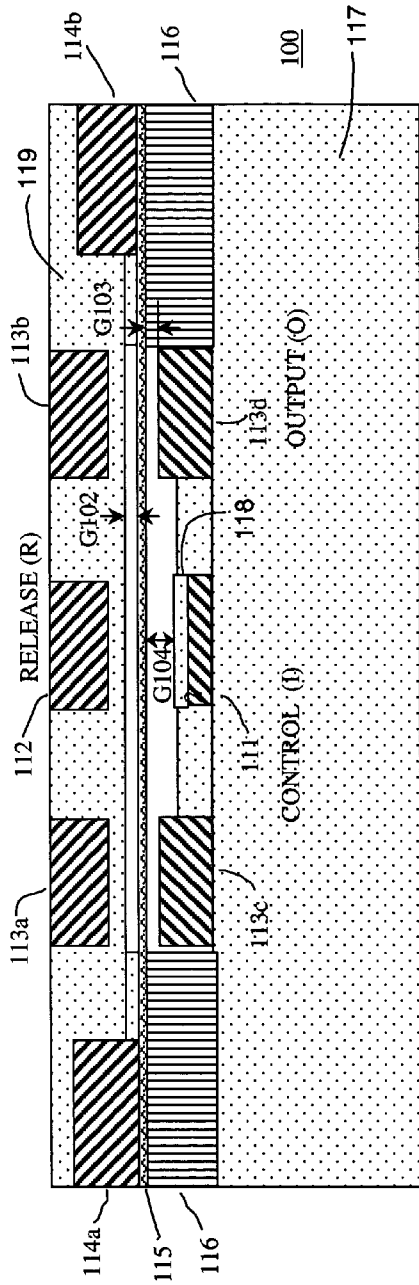
Figure 1A: NT Device Cross Section - Suspended Region
