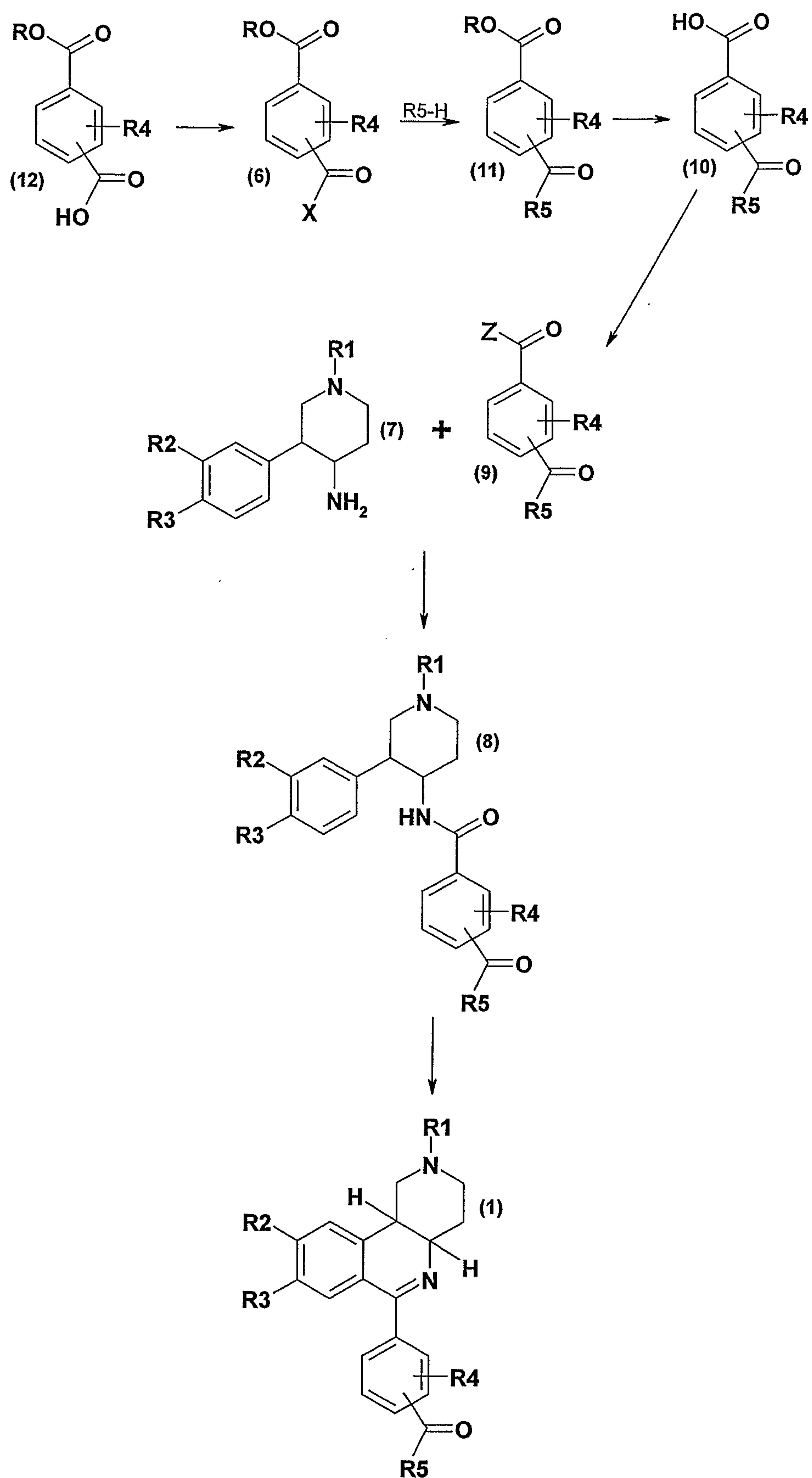
Reaction scheme 2:
