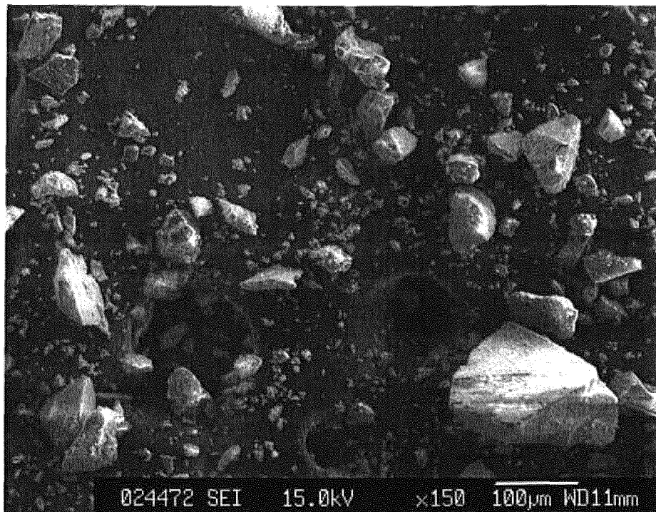
SEM photograph of original raw material (150 times)
