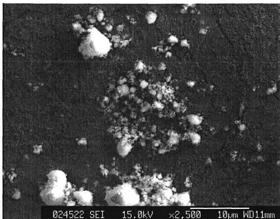
SEM photograph of 3-week-pulverized raw material (2500 times)
