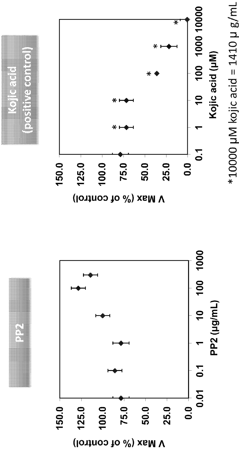
Fig.15 Effect of PP-2 and KA on human tyrosinase (DOPA oxidation) activity in vitro .
