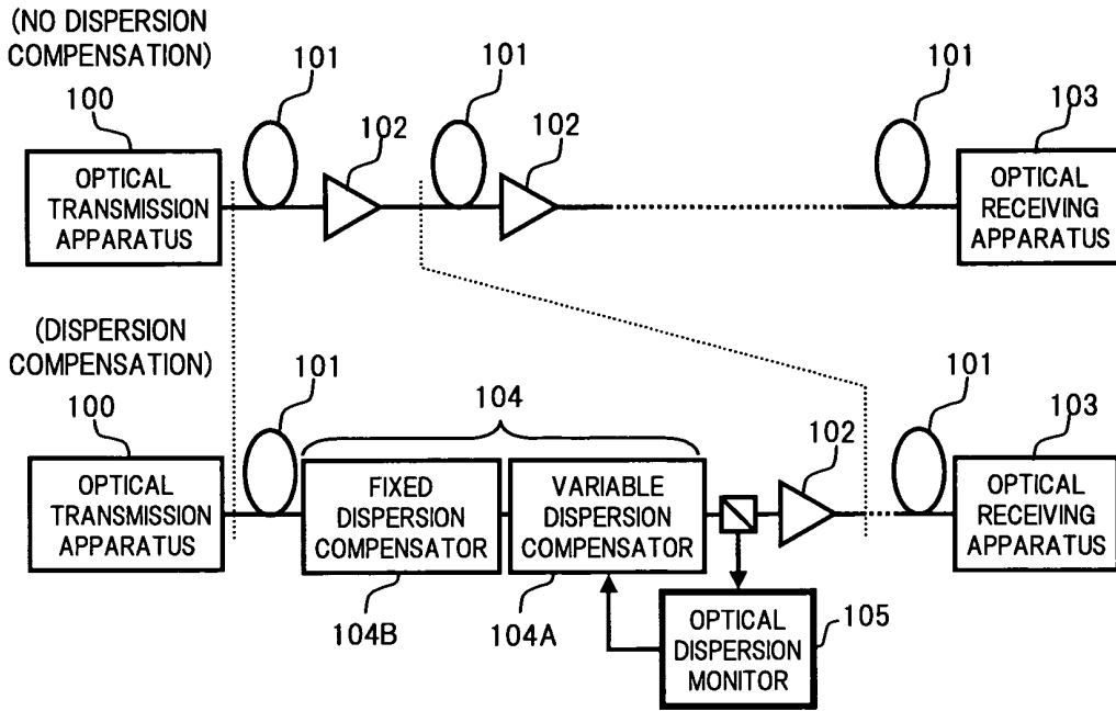
FIG.17 RELATED ART
