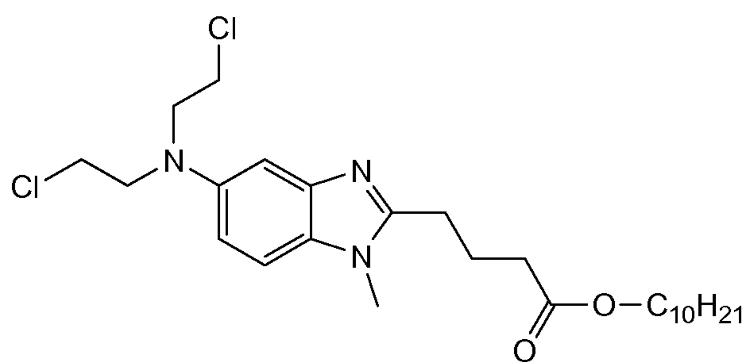
bendamustine C 10 ester
