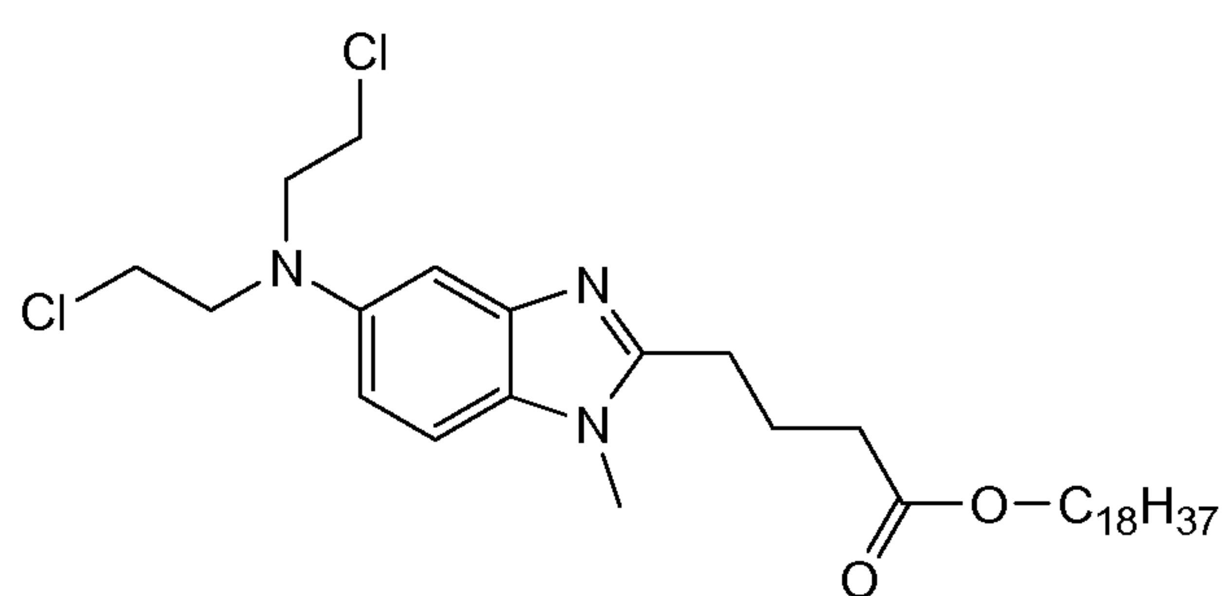
bendamustine C 18 ester
