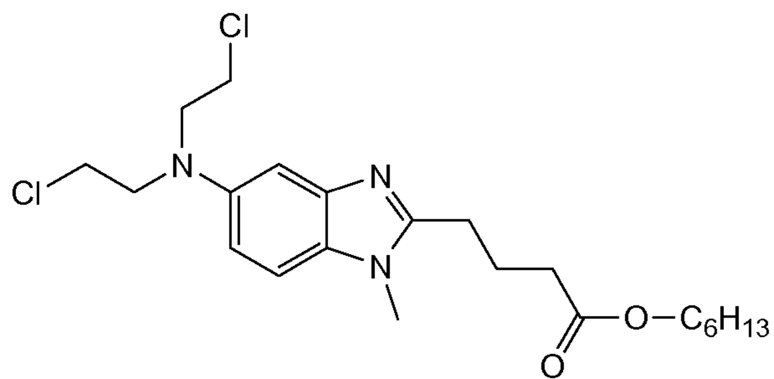
bendamustine C 6 ester
