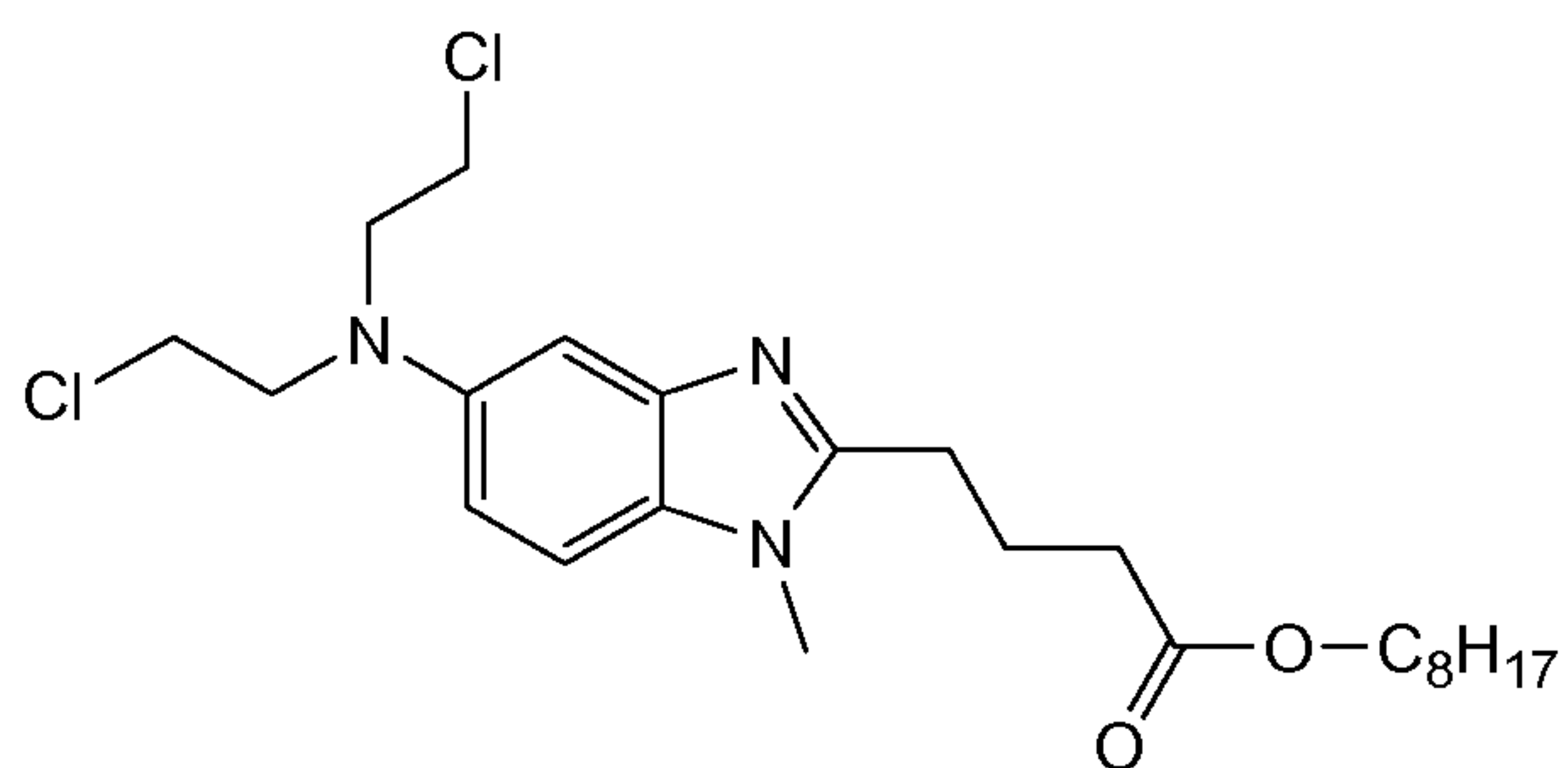
bendamustine C 8 ester
