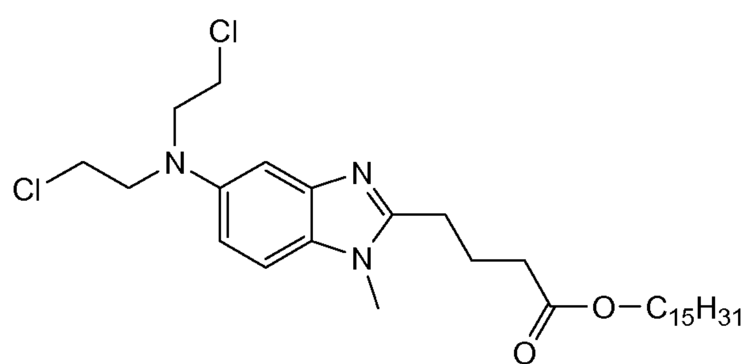
bendamustine C 15 ester
