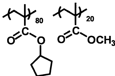
Structural Formula (6)
