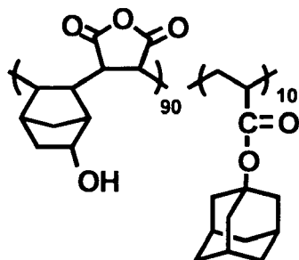
Structural Formula (2)
