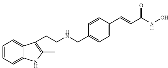
(2E)-N-hydroxy-3-[4-({[2-(2-methyl-1H-indol-3-yl)ethyl]amino}methyl)phenyl]acrylamide
