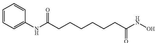
N-hydroxy-M-phenyl-octanediamide
