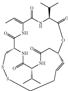
(1S,4S,7Z,10S,16E,21R)-7-ethylidene-4,21-di(propan-2-yl)-2-oxa-12,13-dithia-5,8,20,23-tetrazabicyclo[8.7.6]tricos-16-ene-3,6,9,19,22-pentone
