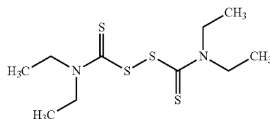
1,1',",1'''-[disulfanediy]bis(carbonothioylnitrilo) tetraethane
