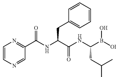
[(1R)-3-methyl-1-({(2S)-3-phenyl-2-[(pyrazin-2-ylcarbonyl)amino]propanoyl}amino)butyl]boronic acid
