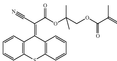
2-(2-cyano-2-(9H-thioxanthen-9-ylidene)acetamido)-2-methylpropyl methacrylate
