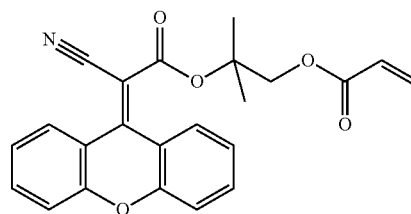
2-(2-cyano-2-(9H-xanthen-9-ylidene)acetoxyl)-2-methylpropyl acrylate
