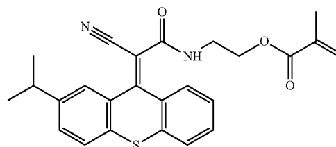
(E)-2-(2-cyano-2-(2-isopropyl-9H-thioxanthen-9-ylidene) acetamido)ethyl methacrylate
