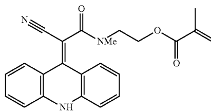
2-(2-(acridin-9(10H)-ylidene)-2-cyano-N-methylacetamido)ethyl methacrylate
