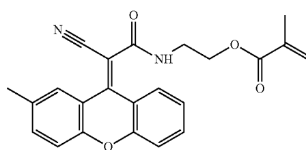
(E)-2-(2-cyano-2-(2-methyl-9H-xanthen-9-ylidene) acetamido)ethyl methacrylate
