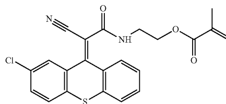
(E)-2-(2-(2-chloro-9H-thioxanthen-9-ylidene)-2- cyanoacetamido)ethyl methacrylate
