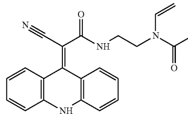
2-(acridin-9(10H)-ylidene)-2-cyano-N-(2-(N-vinylacetamido)ethyl)acetamide
