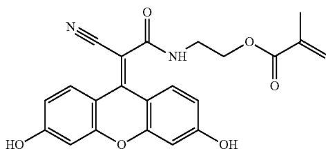
2-(2-cyano-2-(3,6-dihydroxy-9H-xanthen-9-ylidene) acetamido)ethyl methacrylate
