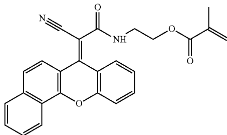
(E)-2-(2-(7H-benzo[c]xanthen-7-ylidene)-2- cyanoacetamido)ethyl methacrylate
