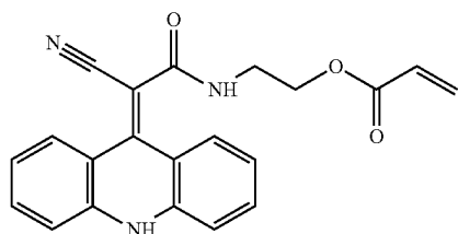
2-(2-(acridin-9(10H)-ylidene)-2-cyanoacetamido)ethyl acrylate
