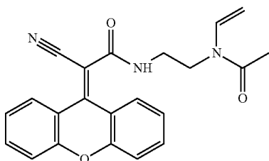
2-cyano-N-(2-(N-vinylacetamido)ethyl)-2-(9H-xanthen-9-ylidene)acetamide
