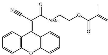
2-(2-cyano-N-methyl-2-(9H-xanthen-9-ylidene)acetamido)ethyl methacrylate
