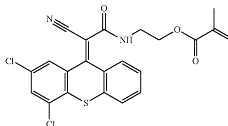
(E)-2-(2-cyano-2-(2,4-dichloro-9H-thioxanthen-9-ylidene) acetamido)ethyl methacrylate
