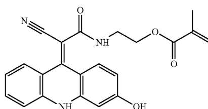
(Z)-2-(2-cyano-2-(3-hydroxyacridin-9(10H)-ylidene)acetamido)ethyl methacrylate
