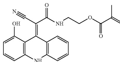
(E)-2-(2-cyano-2-(1-hydroxy-9H-xanthen-9-ylidene) acetamido)ethyl methacrylate
