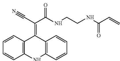
N-(2-(2-(acridin-9(10H)-ylidene)-2-cyanoacetamido)ethyl)acrylamide
