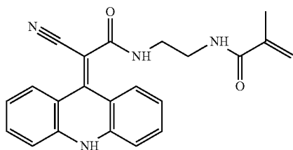
N-(2-(2-(acridin-9(10H)-ylidene)-2-cyanoacetamido)ethyl)methacrylamide
