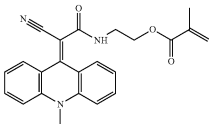
2-(2-cyano-2-(10-methylacridin-9(10H)-ylidene) acetamido)ethyl methacrylate
