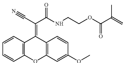
(Z)-2-(2-cyano-2-(3-methoxy-9H-xanthen-9-ylidene) acetamido)ethyl methacrylate
