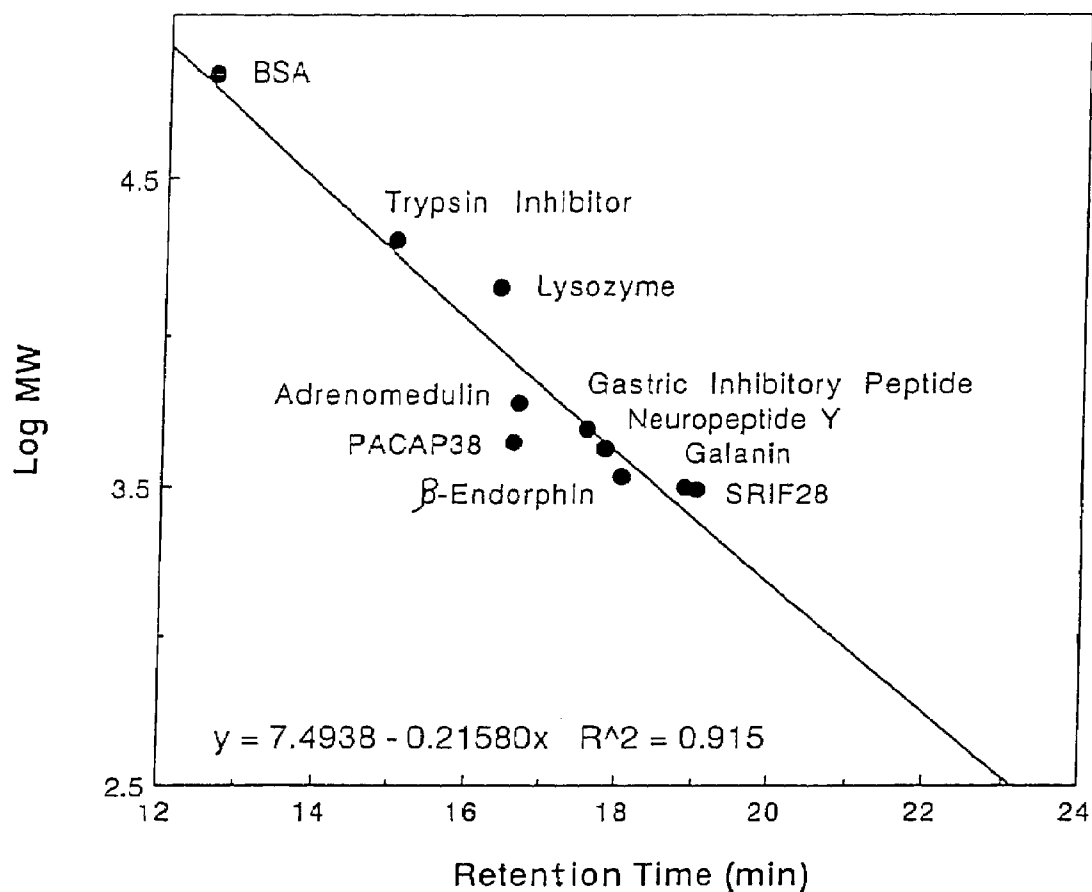
G2000SWXL Calibration
