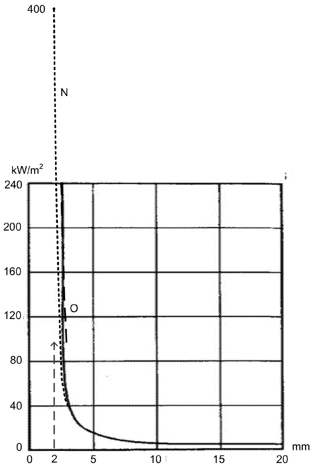
Figure 3 (Prior Art)
