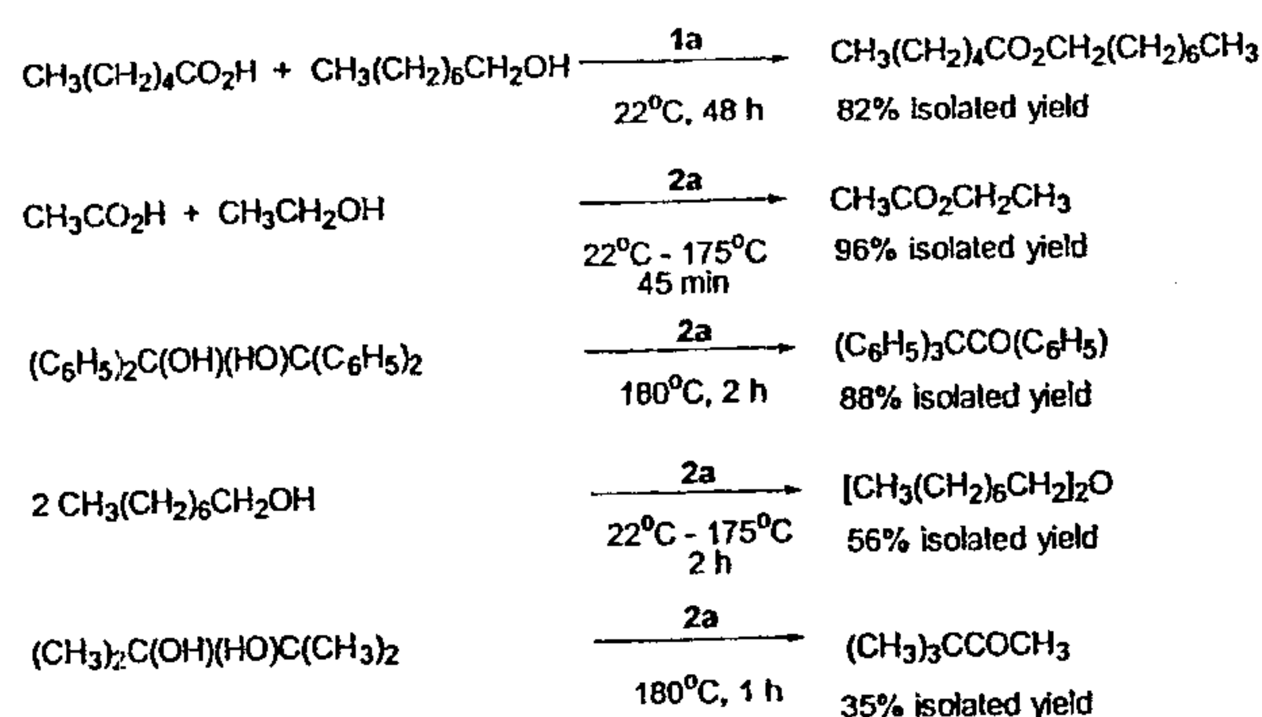
Scheme 1. Representative reactions using IL 1a and 2a .
