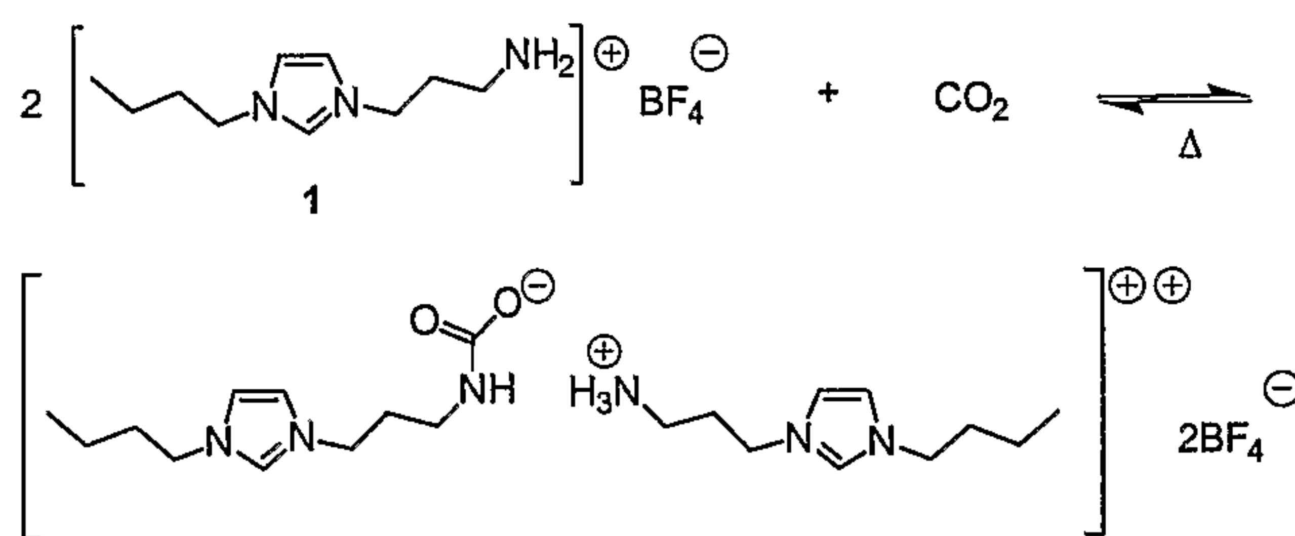
Scheme 2. Proposed reaction between TSIL 1 and CO 2 .
