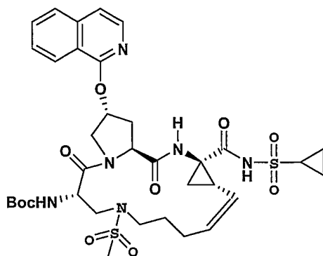
Compound 153
