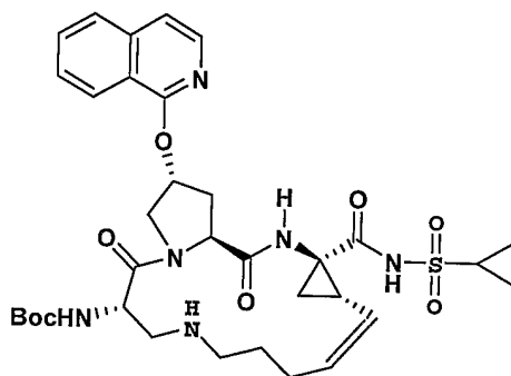
Compound 151
