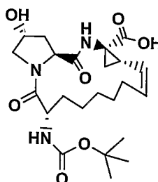
Example 20
