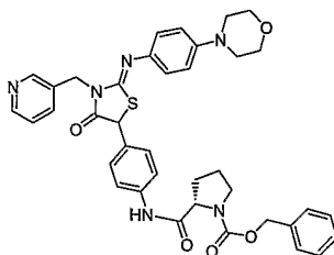
NS5A Inhibitor
