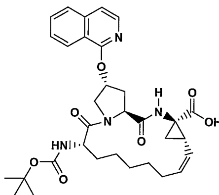
Example 2, Compound 1
