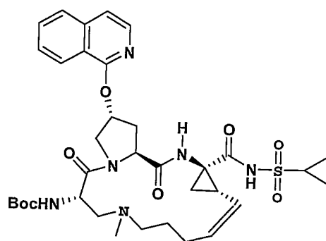
Compound 147
