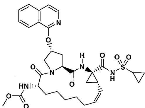
Compound 12
