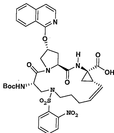
compound 144
