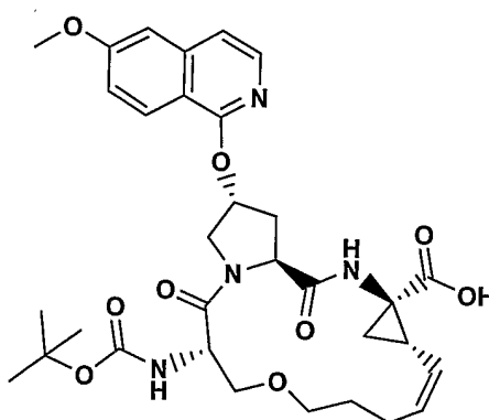
Compound 84
