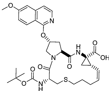
Compound 18A
