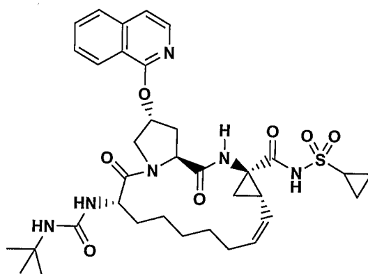
compound 126
