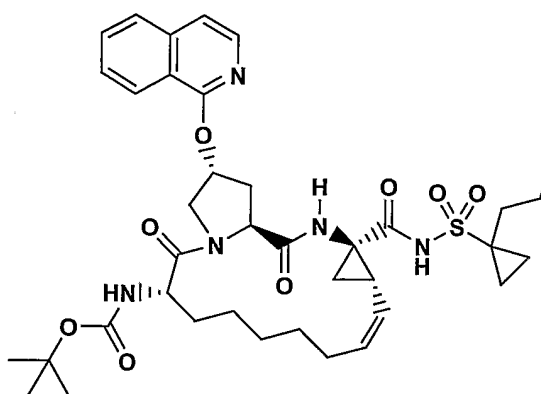
Compound 6
