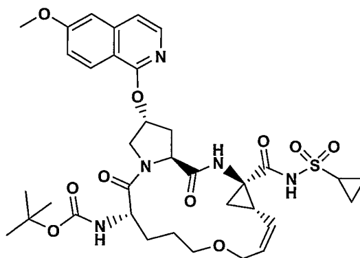
Compound 28
