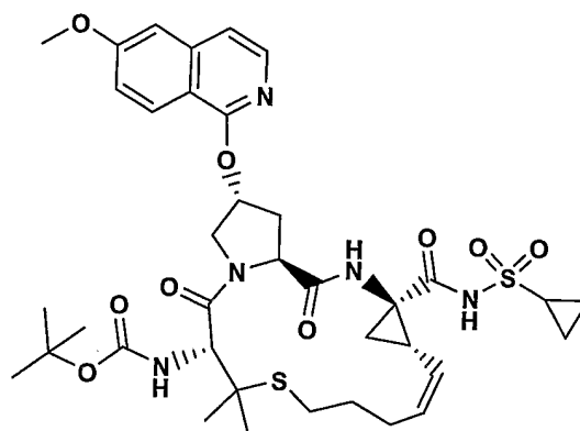
Compound 80
