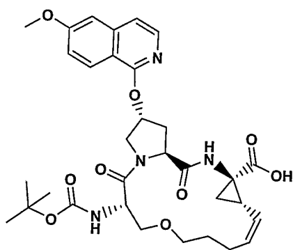
Compound 84
