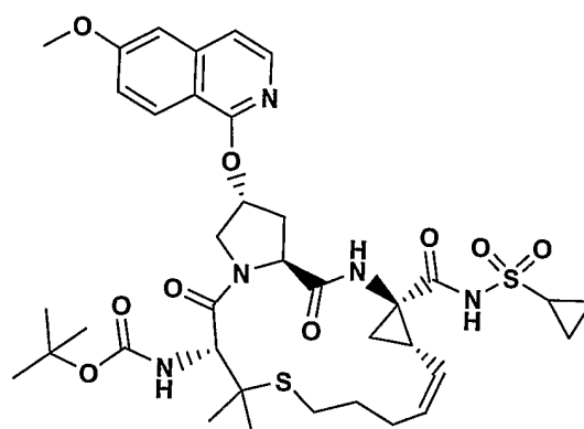
Compound 80
