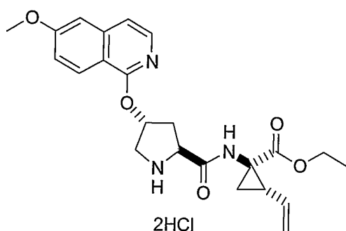
Example 22
