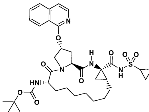
Compound 10
