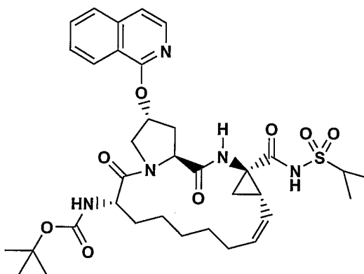
Compound 3
