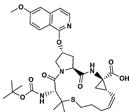
Compound 79
