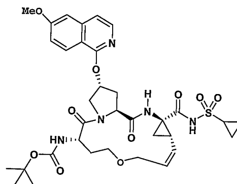
compound 141
