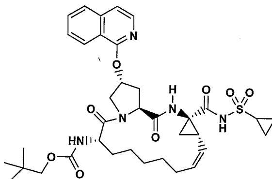
Compound 13
