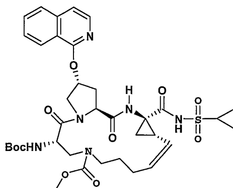
Compound 148
