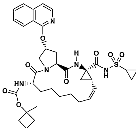
compound 56
