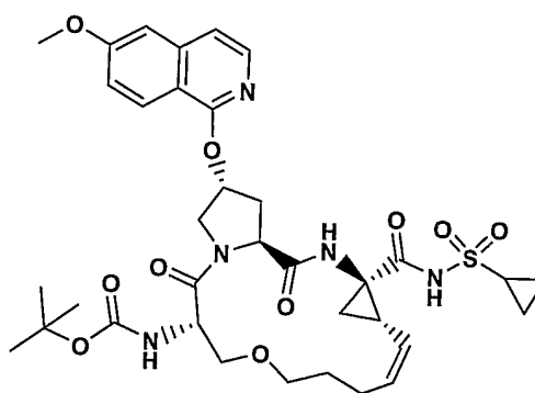
Compound 85
