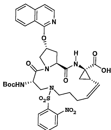
Compound 144
