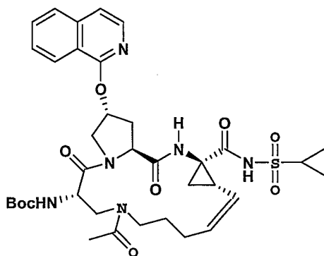
Compound 146
