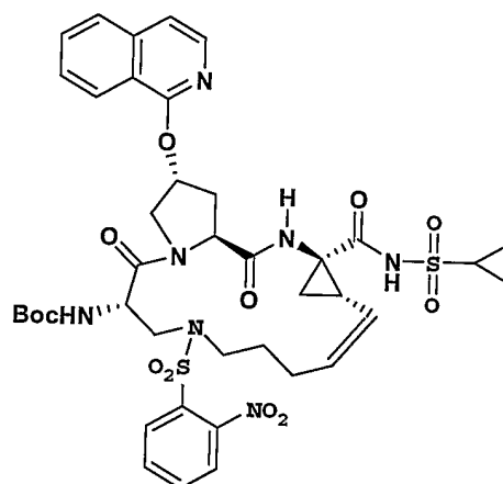
Compound 145
