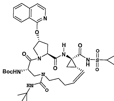
Compound 150
