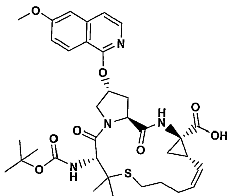
Compound 79
