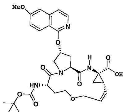
compound 140
