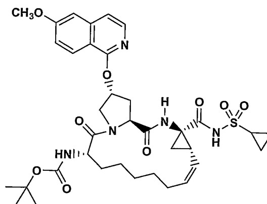
Compound 17B
