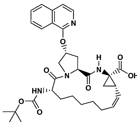
Compound 1
