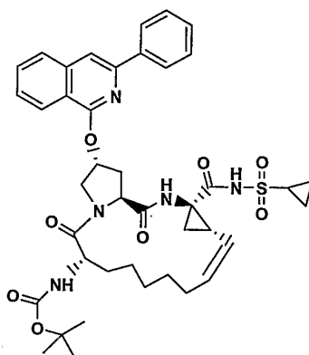
compound 58
