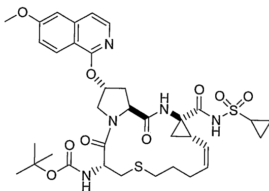
Compound 18B
