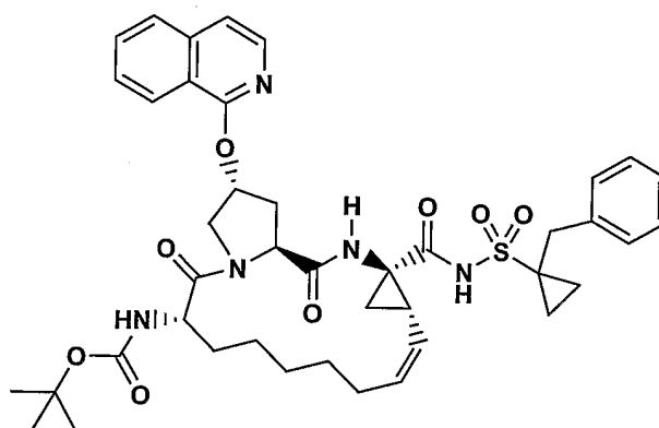
Compound 5
