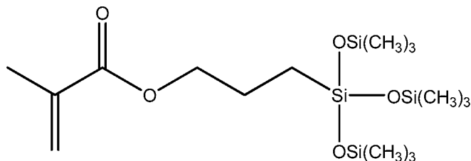
Methacryloxypropyltris(trimethylsiloxy)silane (TRIS)
