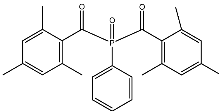
IRGACURE 819 (photoinitiator)
