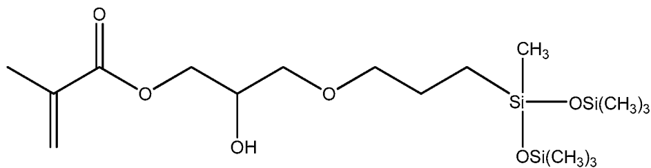
(3-methacryloxy-2-hydroxypropoxy)propyl bis(trimethylsiloxy)methylsilane
