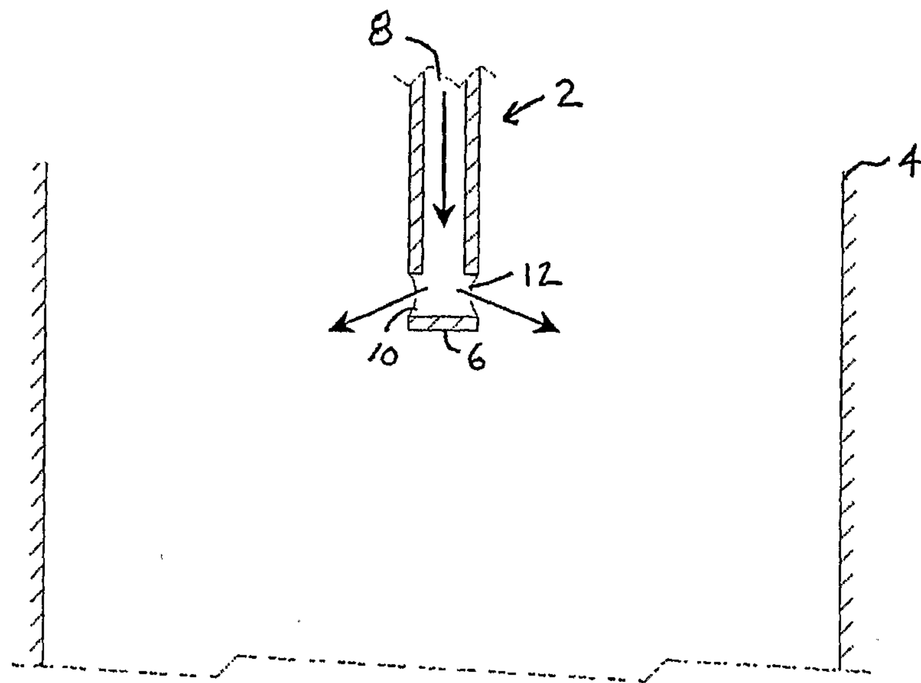
Fig. 1 PRIOR ART
