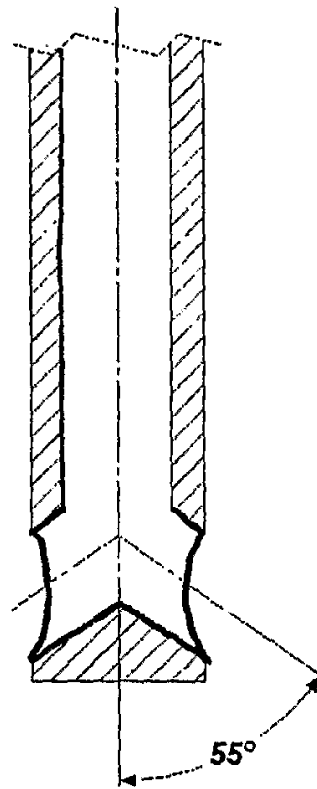
Fig. 3 PRIOR ART
