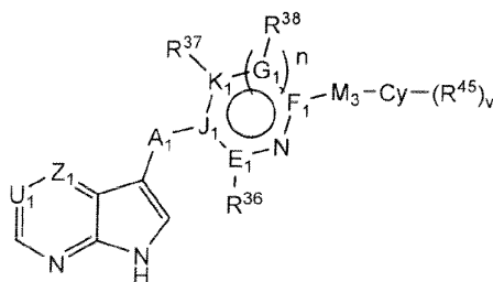
Formula Ig,
