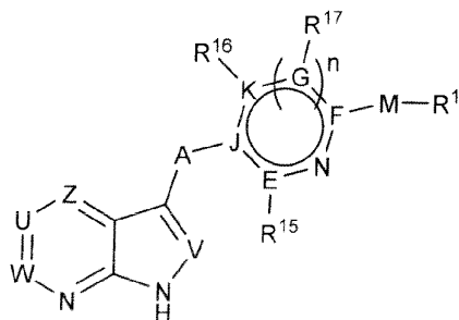
Formula Ib
