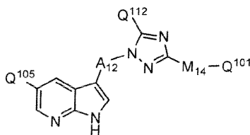
Formula IIk,
