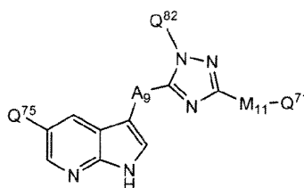
Formula IIh,
