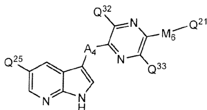
Formula IIc,
