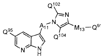
Formula Iij,
