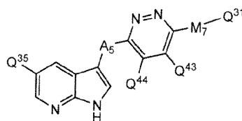
Formula IId,
