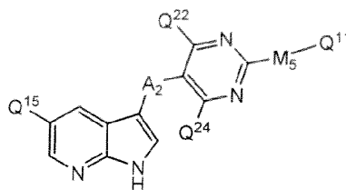
Formula IIb,
