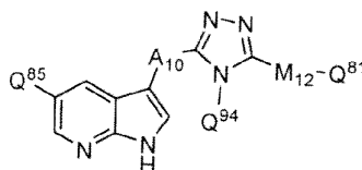
Formula III,
