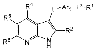
Formula Ia
