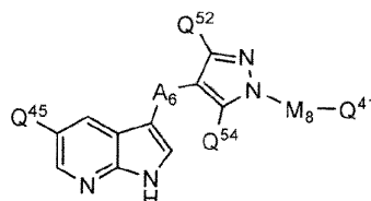
Formula IIe,
