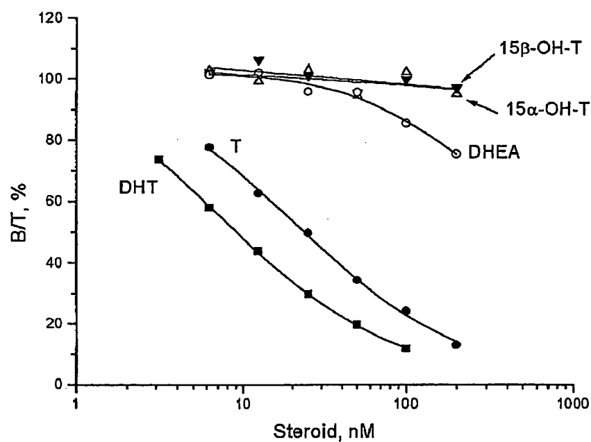
Figure 1: Competition curves showing displacement of [ 3 H]DHT from human SHBG using 5α-dihydrotestosterone (DHT), testosterone (T), dehydroepiandrosterone (DHEA), 15α-hydroxytestosterone (15α-OH-T), 15β-hydroxytestosterone (15β-OH-T) as competitors. Results are expressed as bound (B) cpm at each competitor concentration/total (T) cpm bound in absence of competitor as a percentage.
