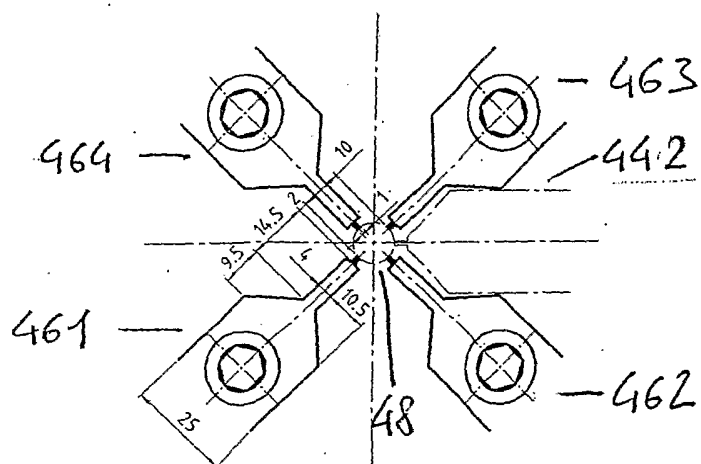
detail Z (1:1) FIG. 11
