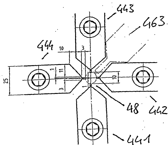
detail Z (1:1) FIG. 11
