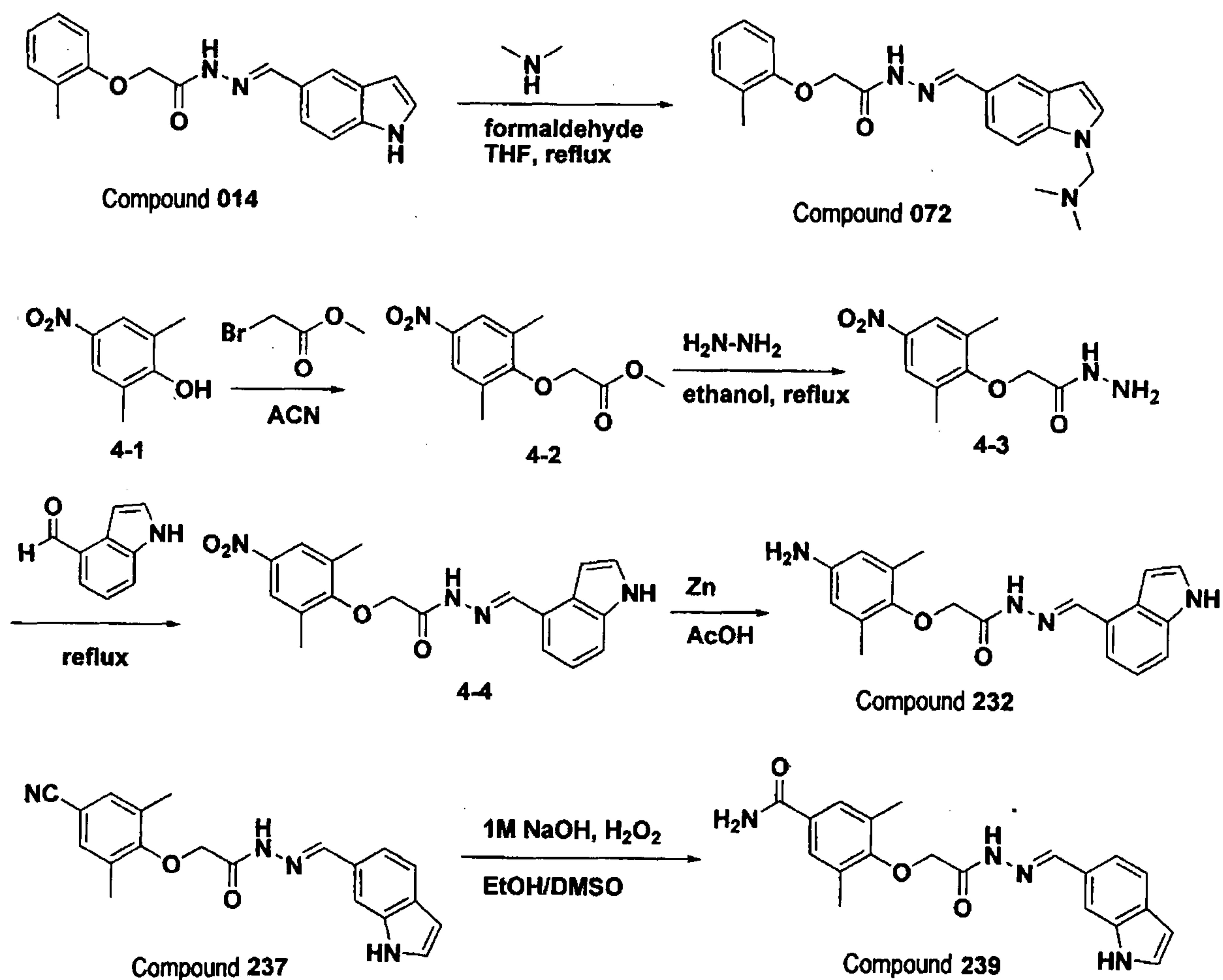
[Scheme 4]
