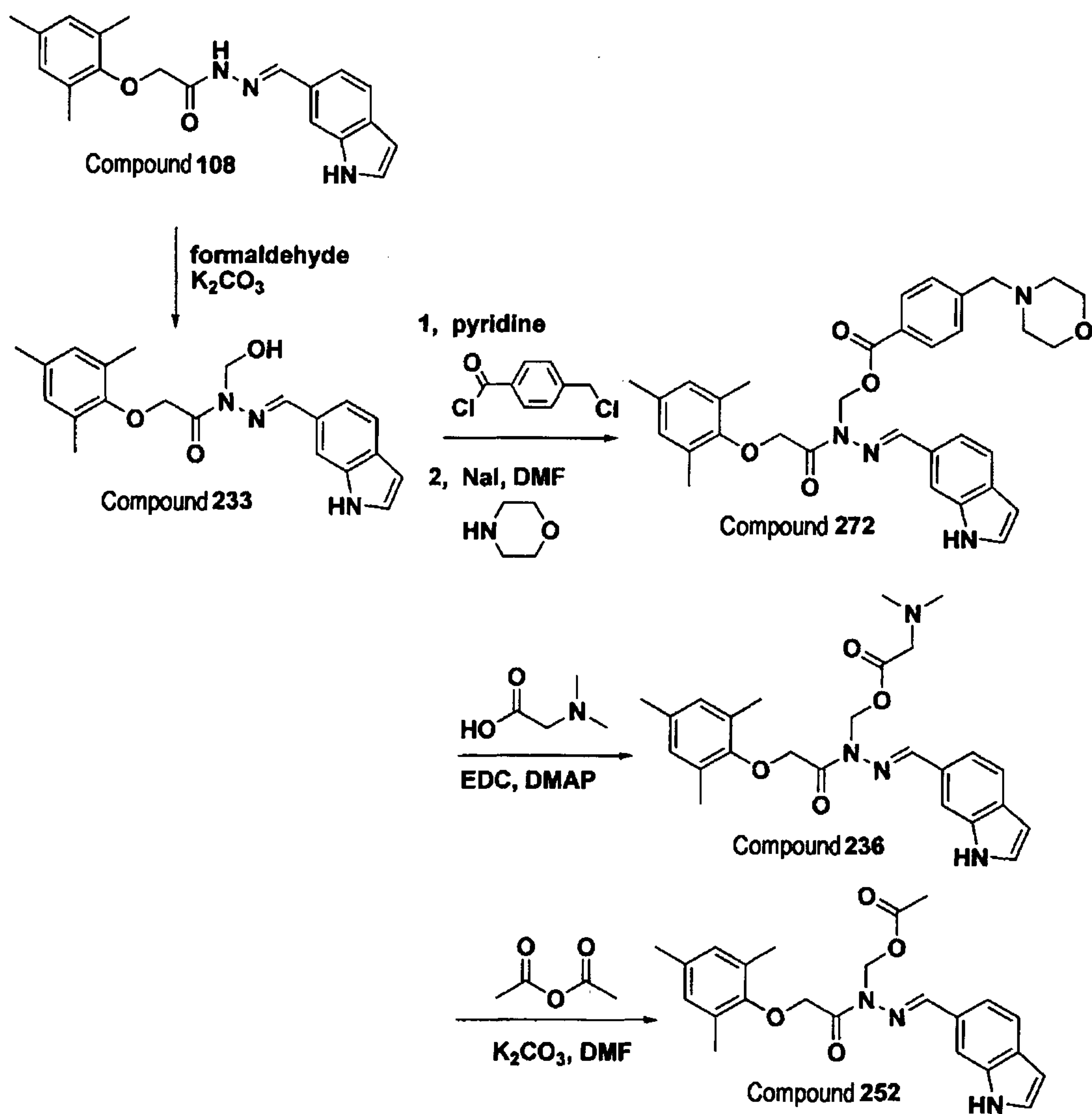
[Scheme 2]
