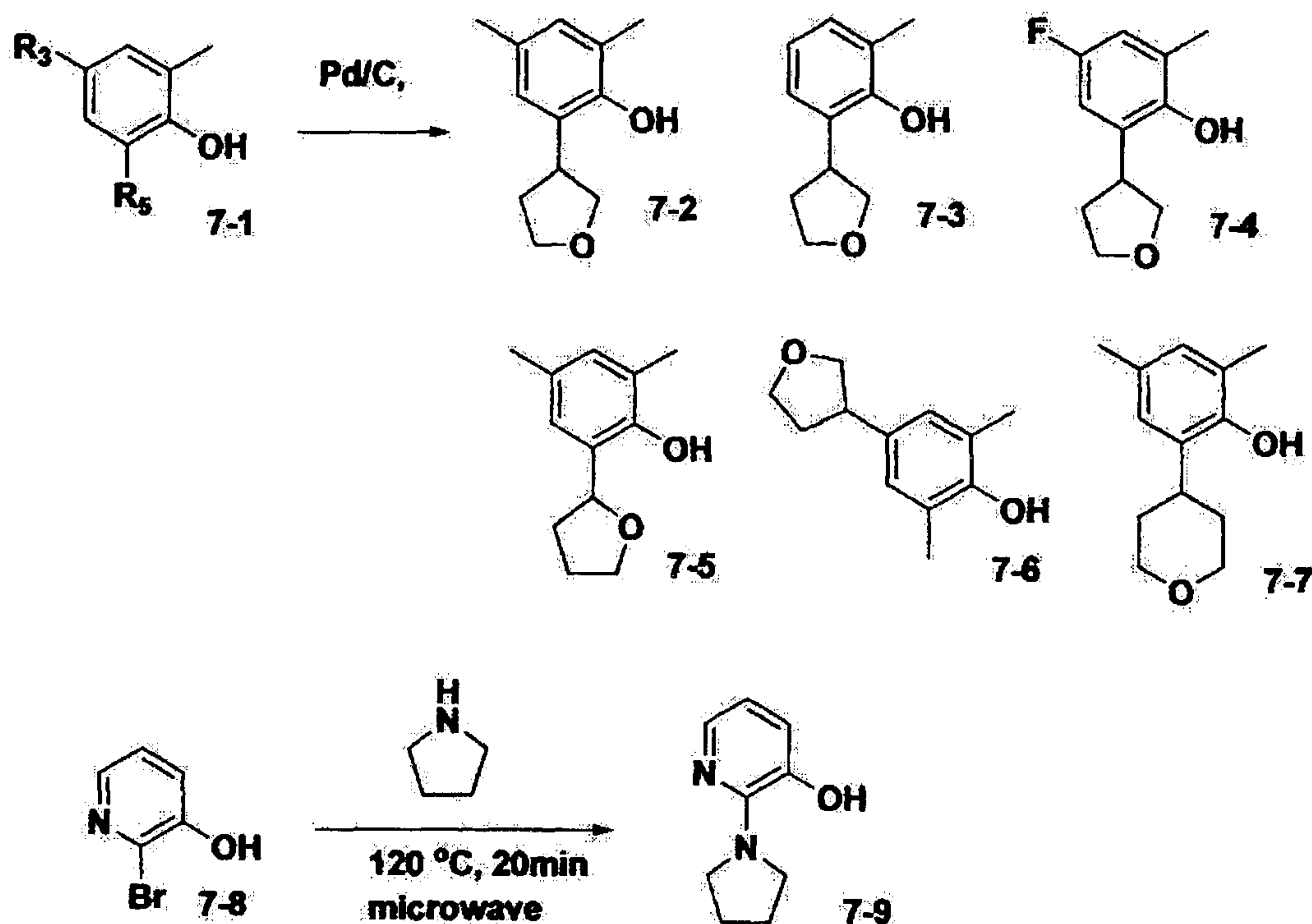
[Scheme 7]
