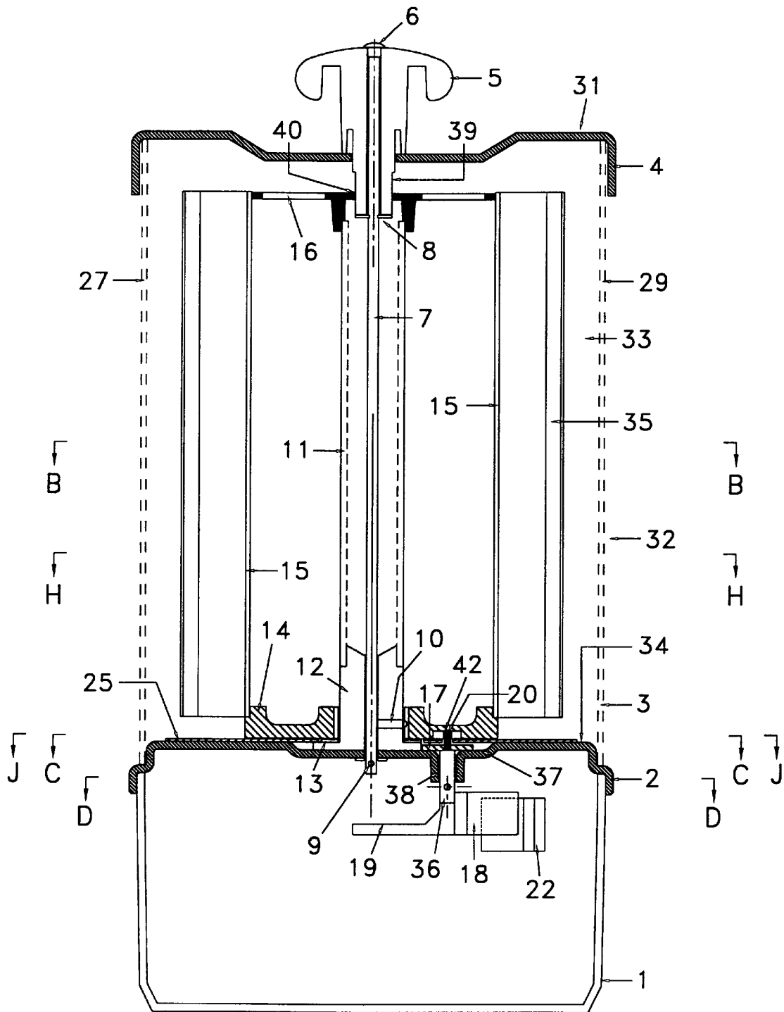
CROSS SECTION "A" - "A"
