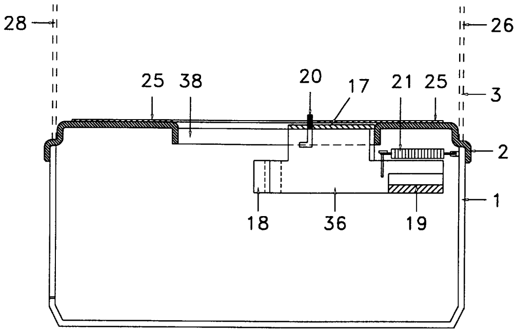
CROSS SECTION "F" - "F"
