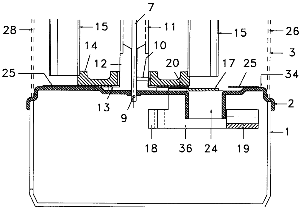
CROSS SECTION "G" - "G"
