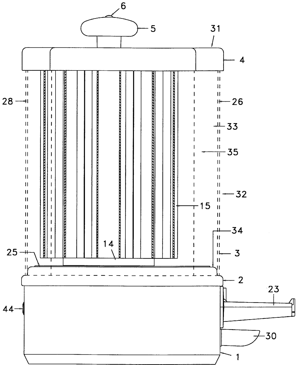
LEFT SIDE VIEW
