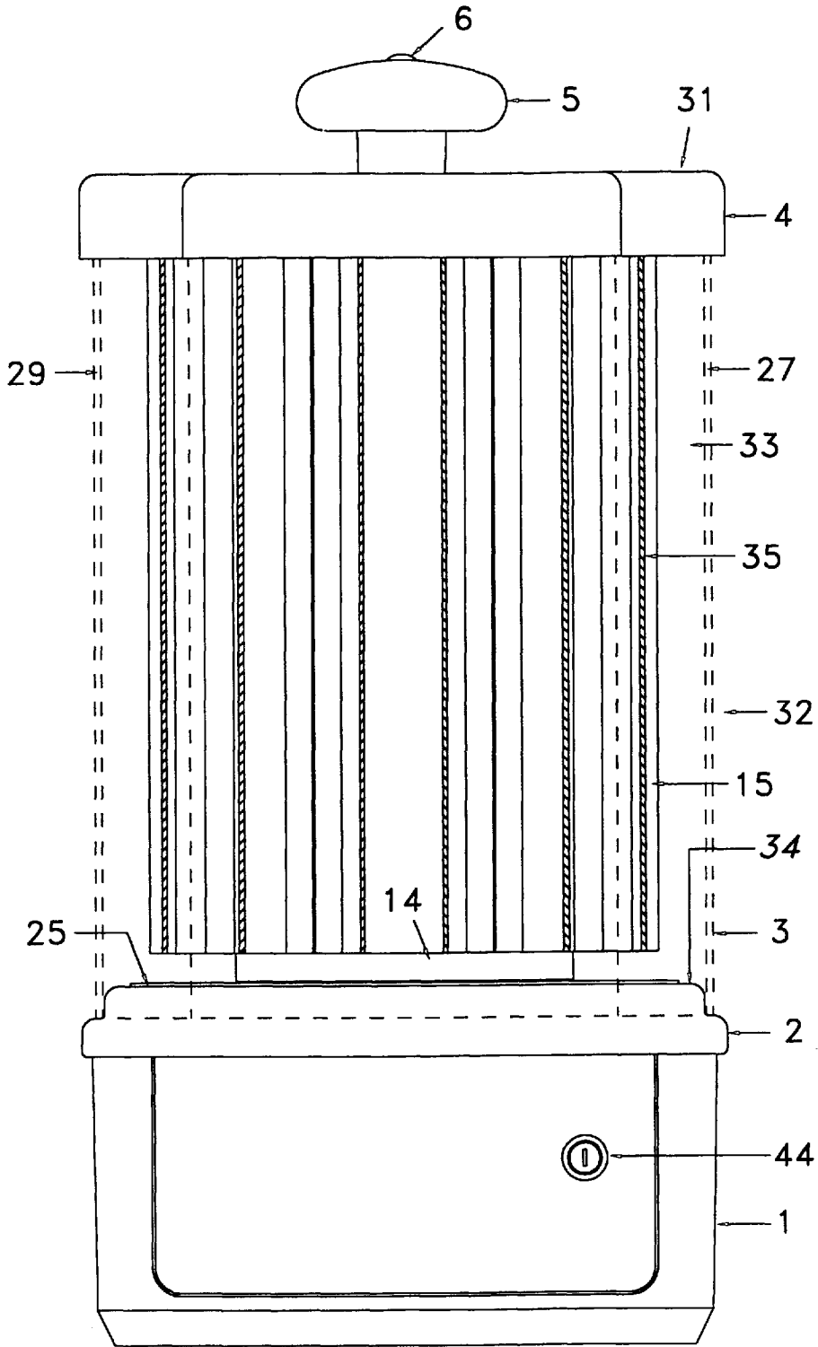
REAR VIEW
