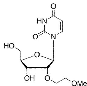
2'-O-methoxyethyl uridine
