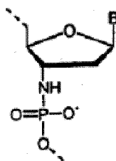
N3'-P5' Phosphoroamidate
