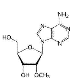
2'-O-methyl-adenosine
