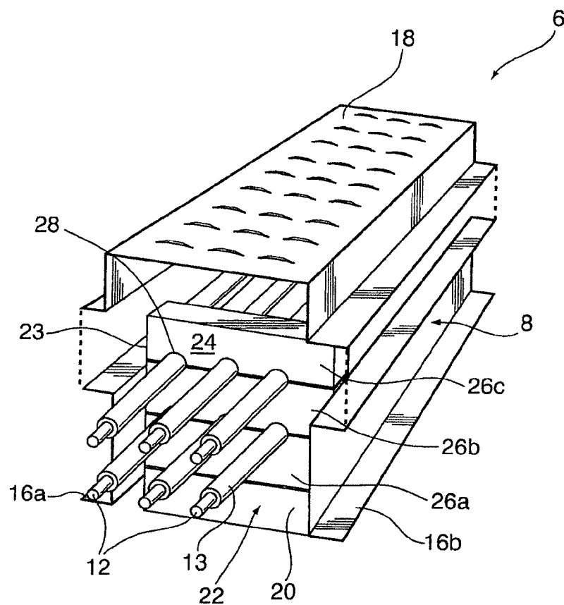
Fig. 1 Prior Art
