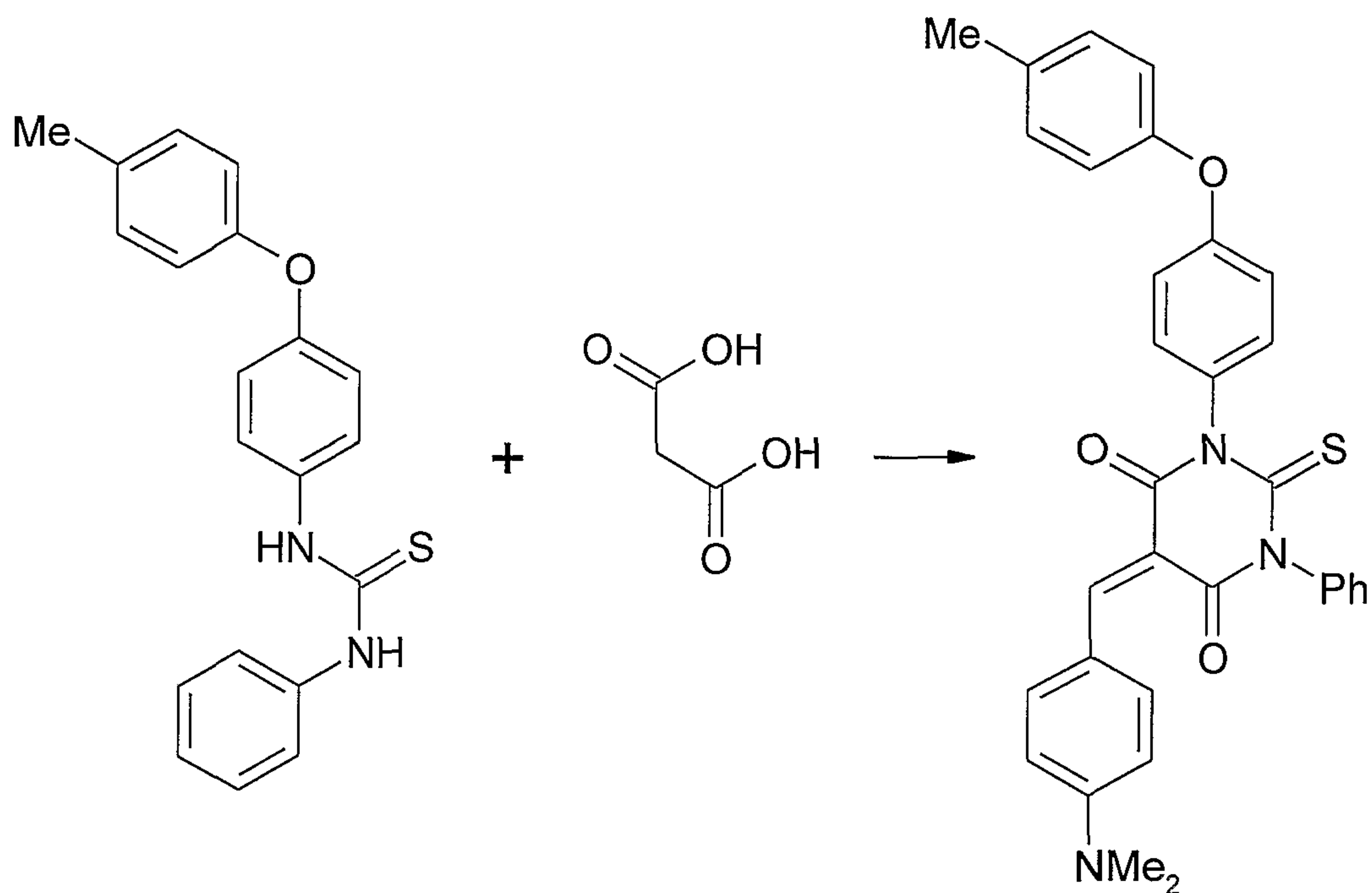
Scheme 17 - Swarup et al., 1991
