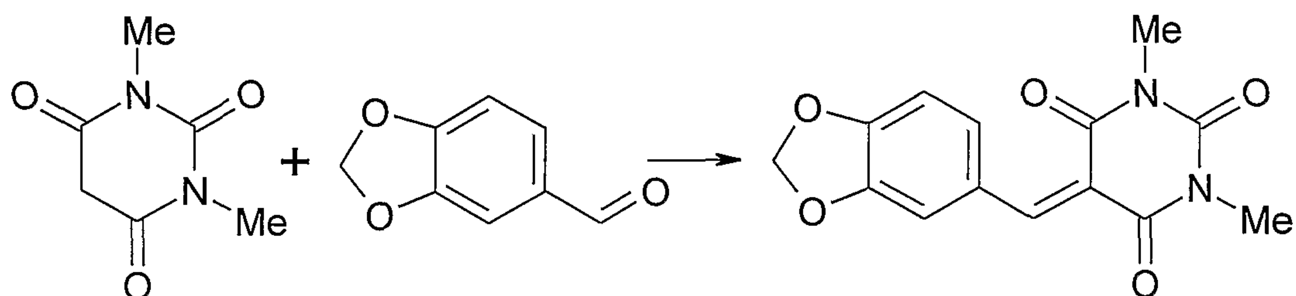
Scheme 7 - Chan et al., 1991
