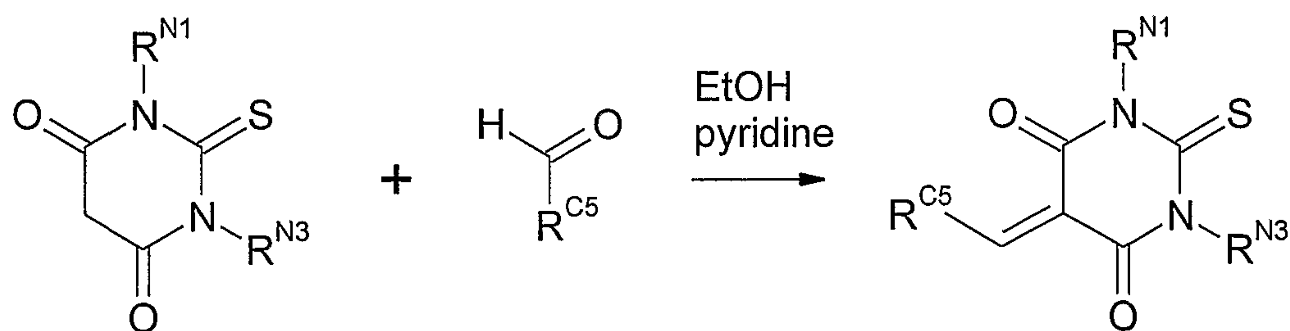
Scheme 16
