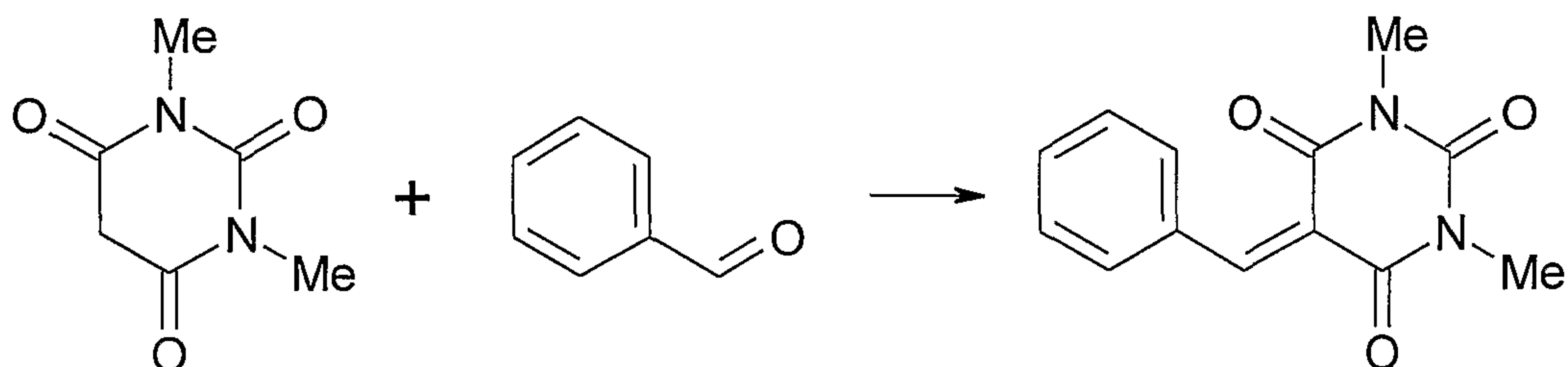
Scheme 6 - Figueroa-Villar et al., 1992
