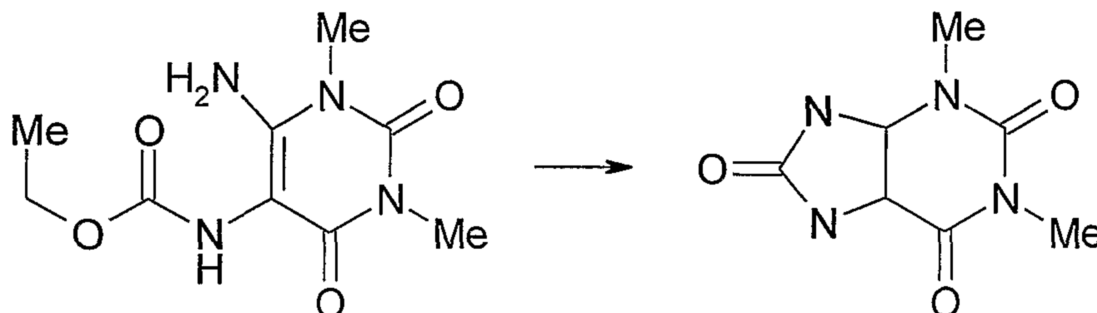
Scheme 20 - Taylor et al., 1974
