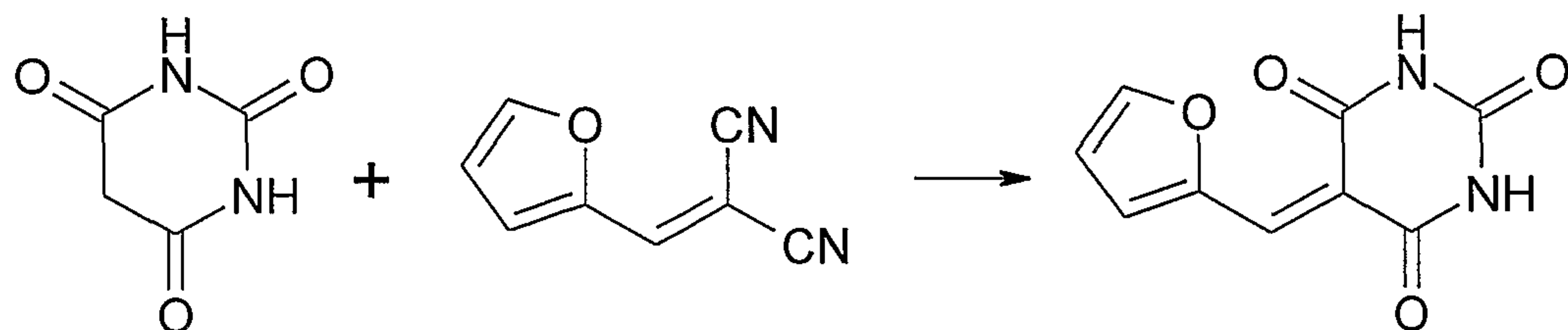
Scheme 10 - Hennig et al., 1992
