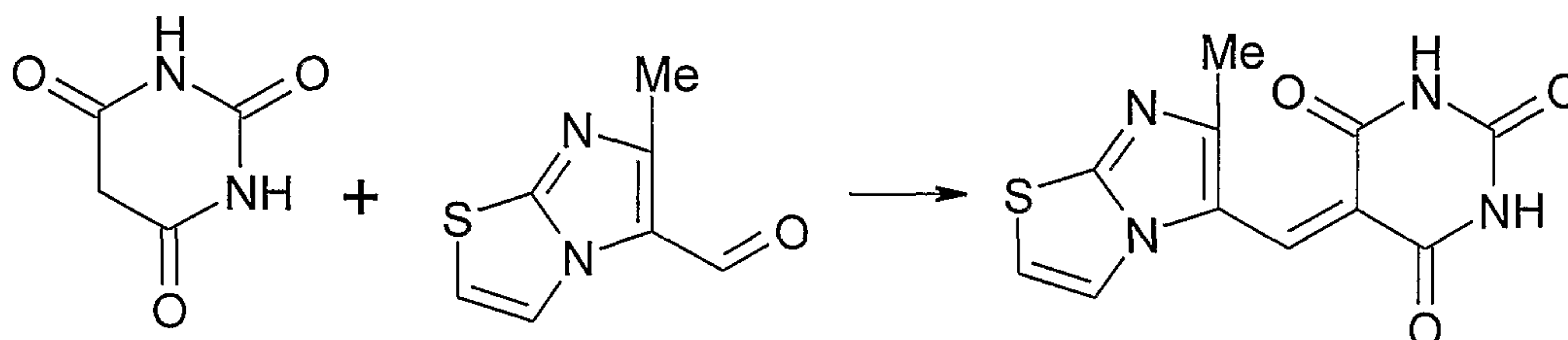
Scheme 3 - Strakov et al., 1996
