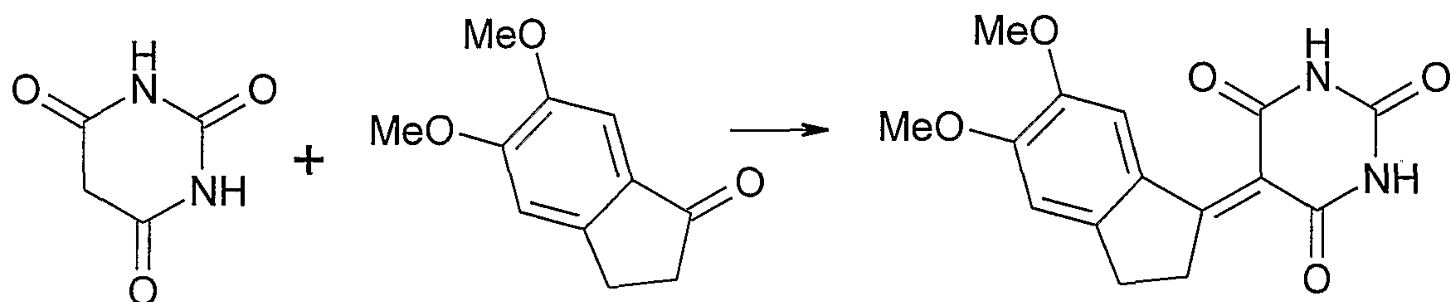
Scheme 8 - Joshi et al., 1990
