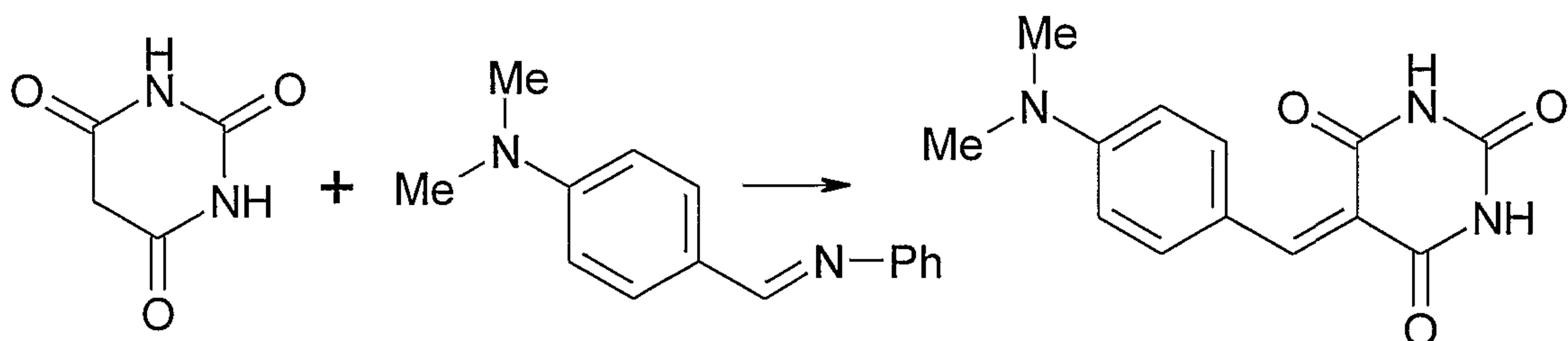
Scheme 10 - Hennig et al., 1992
