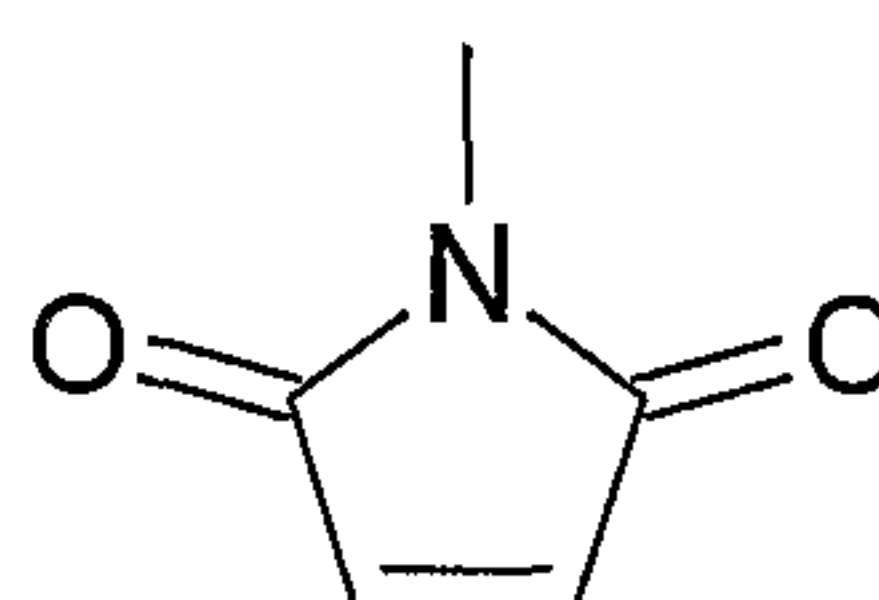
maleimidyl
