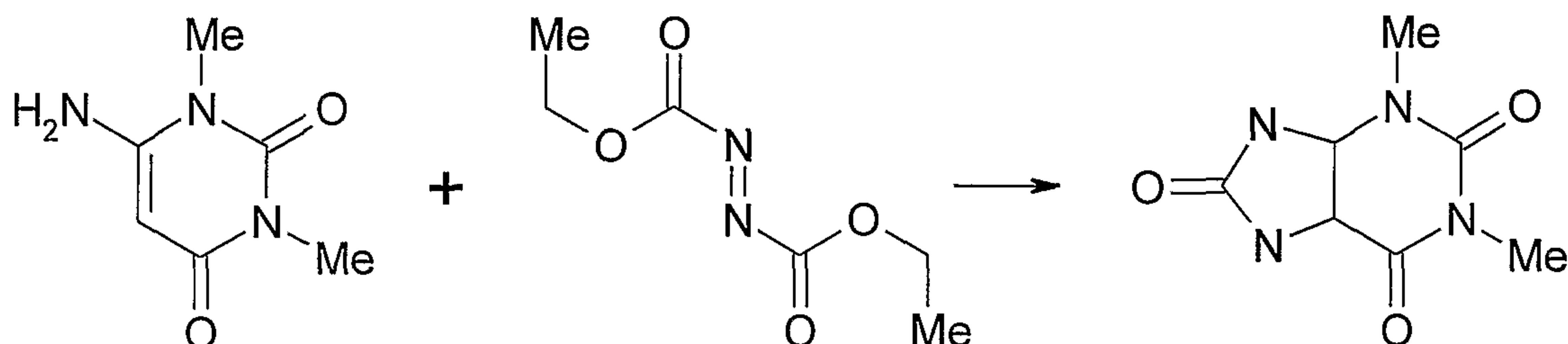
Scheme 20 - Taylor et al., 1974
