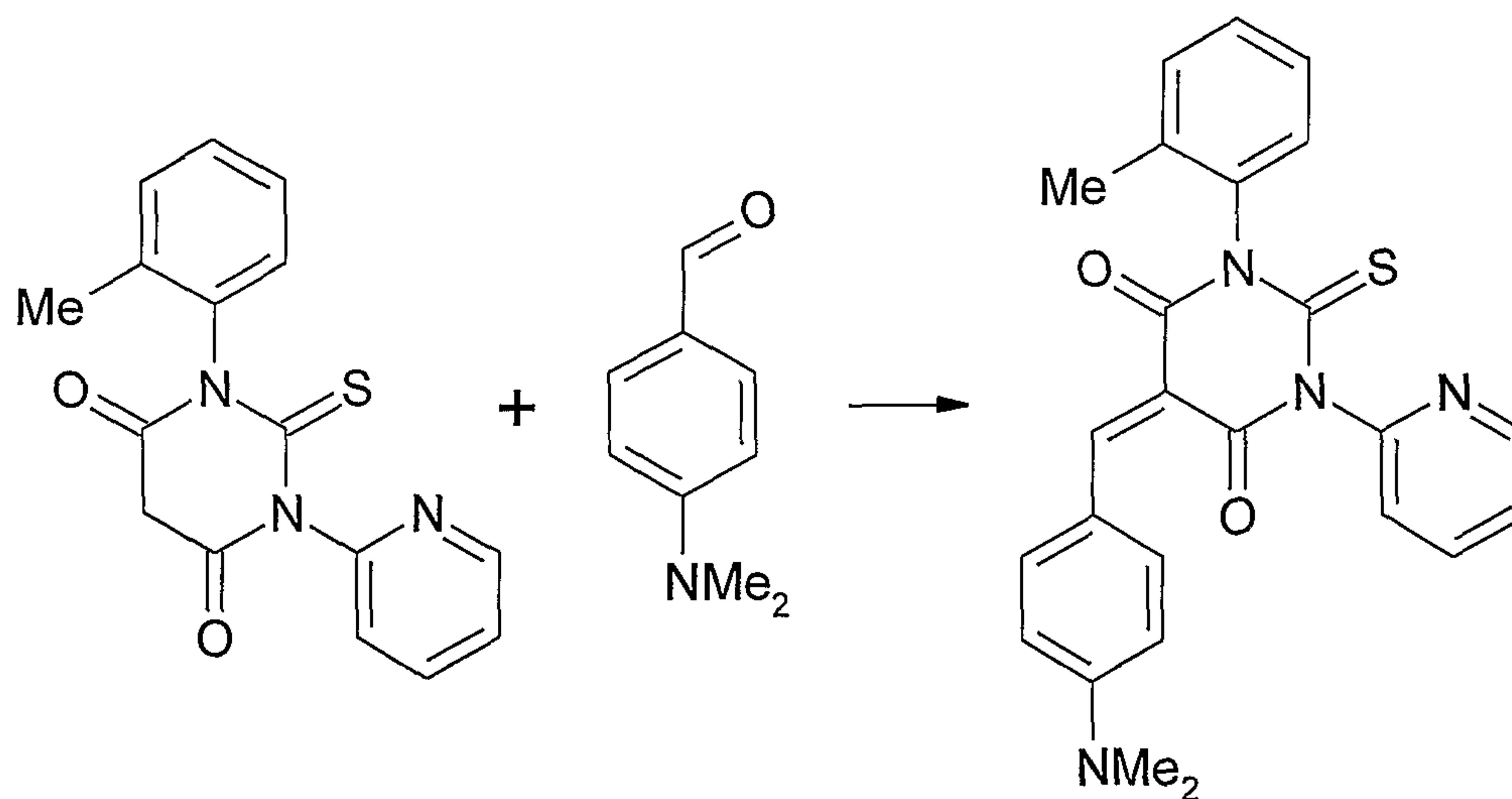
Scheme 14 - Shalmashi et al., 1994
