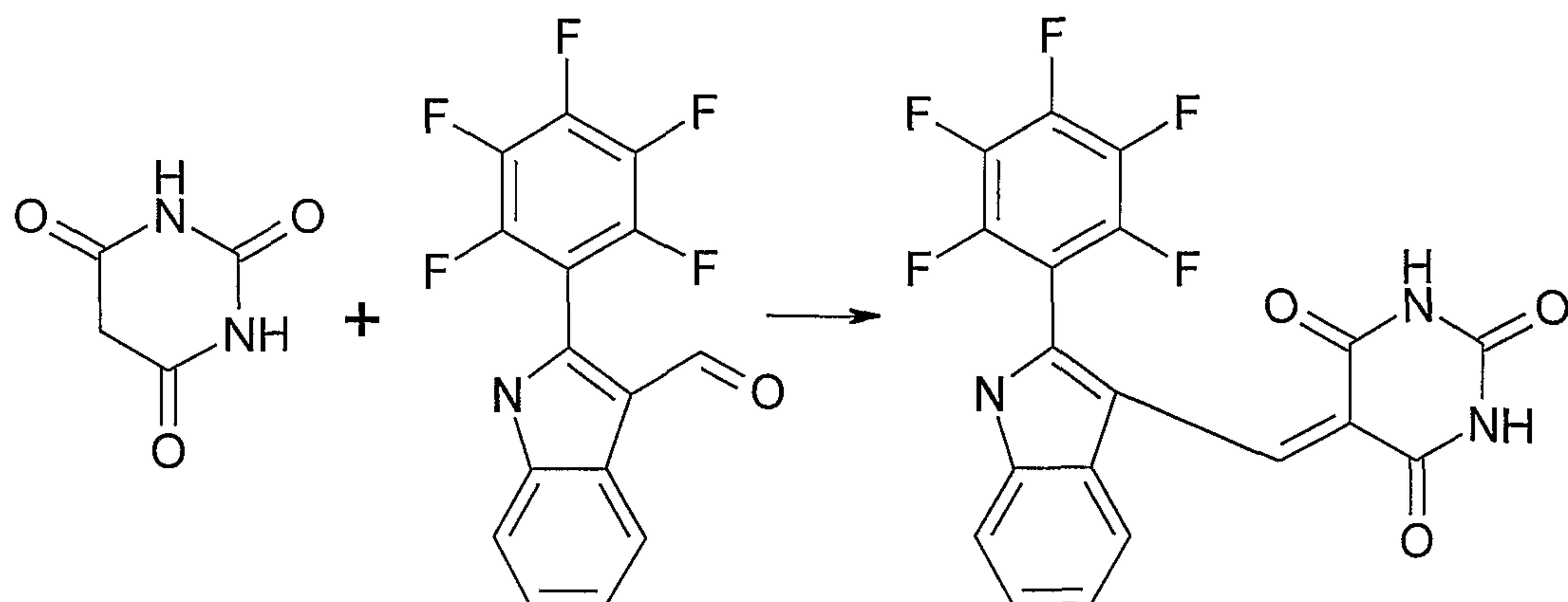
Scheme 8 - Joshi et al., 1990
