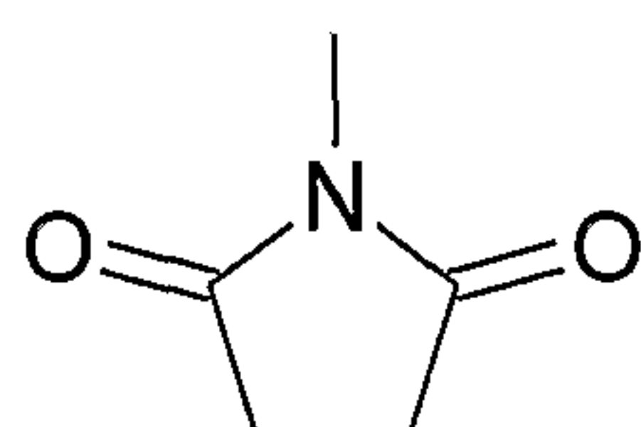
succinimidyl
