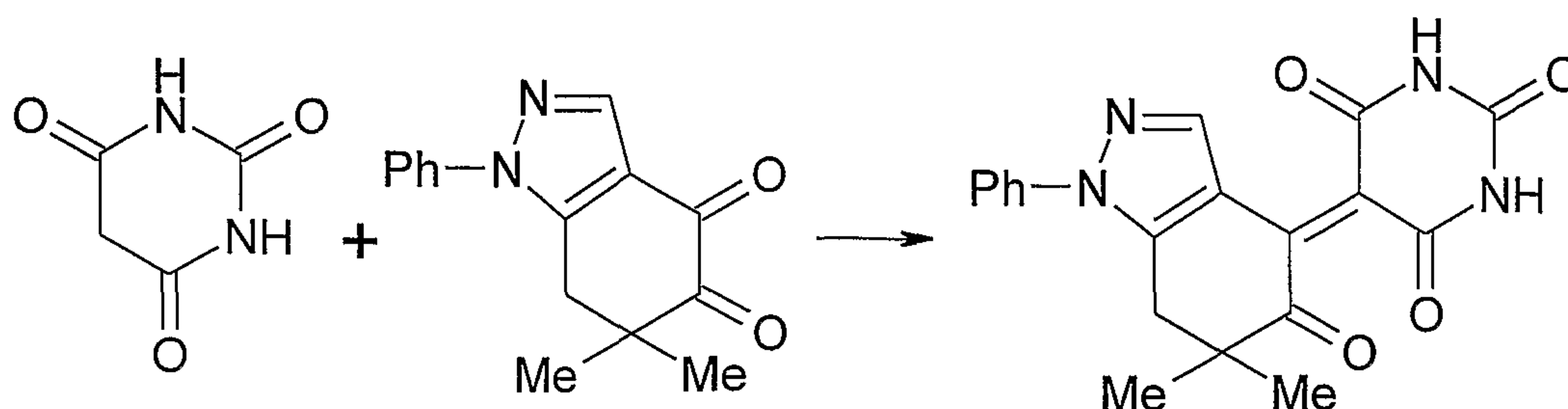
Scheme 3 - Strakov et al., 1996
