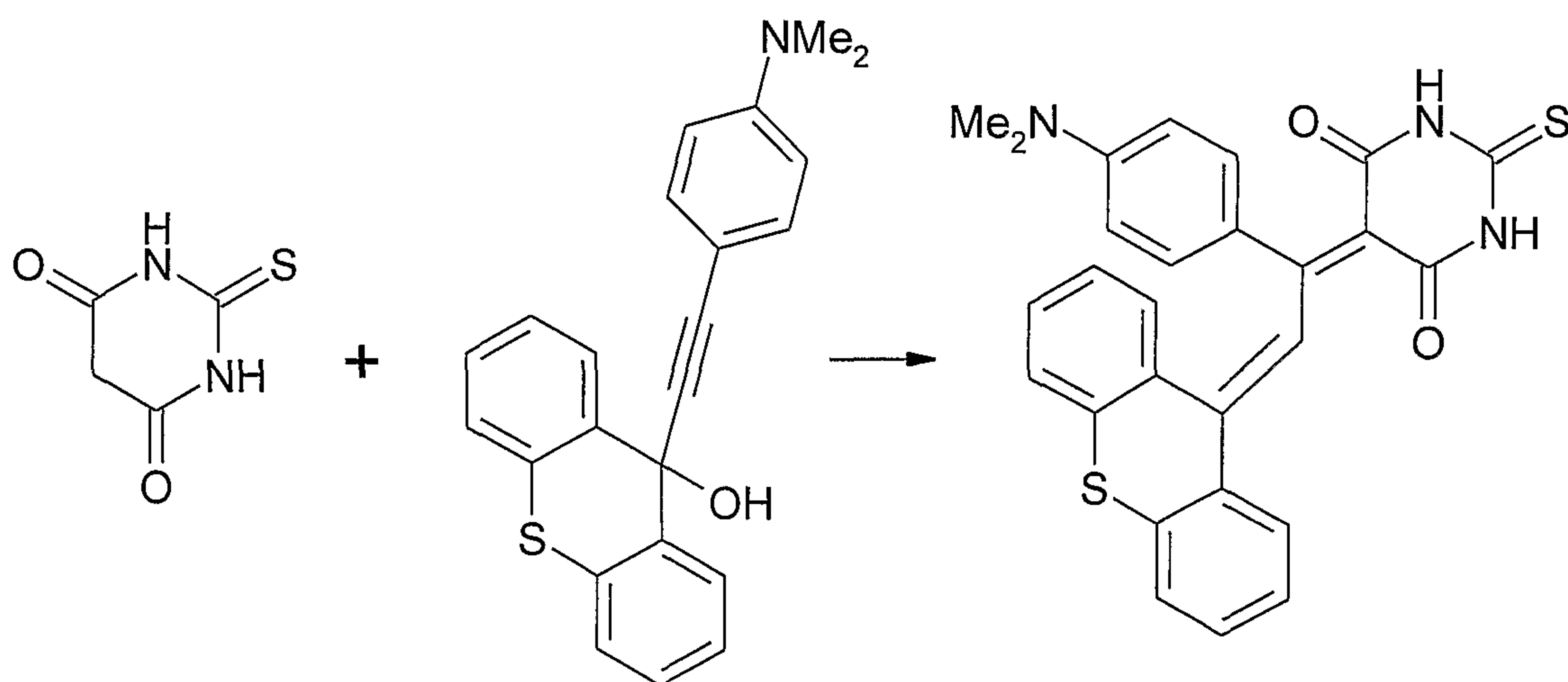
Scheme 18 - Nakatsuji, 1988
