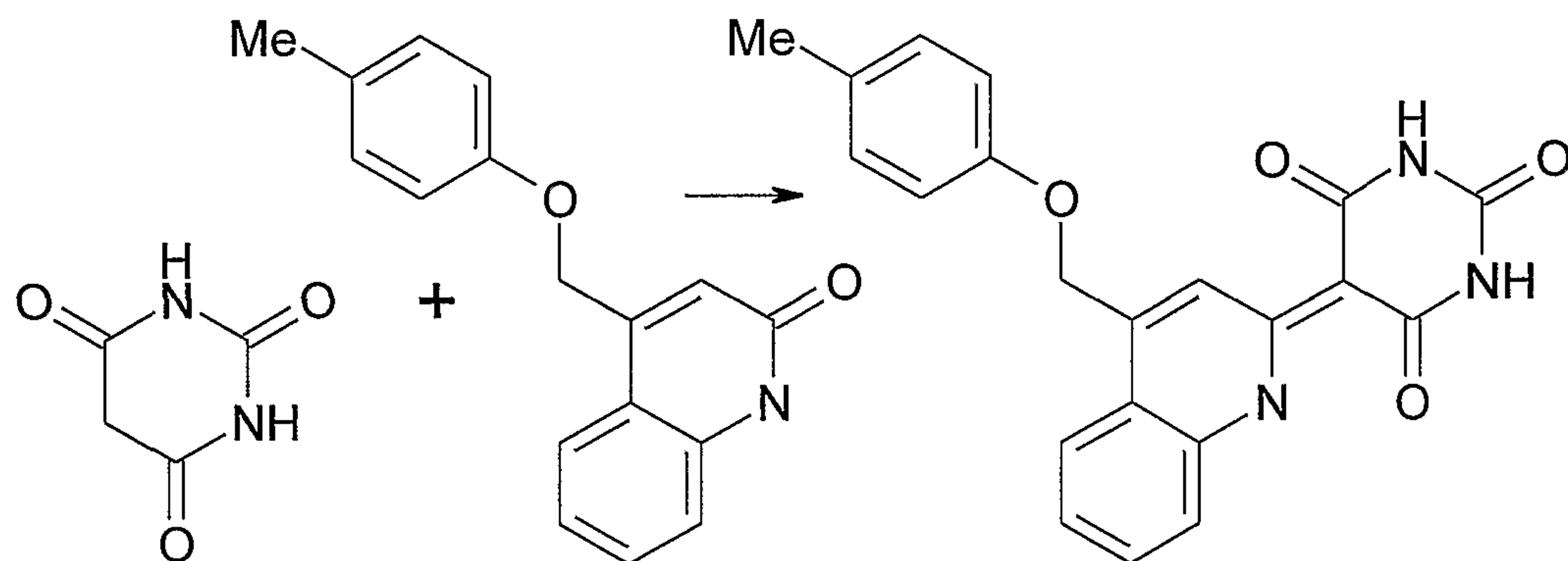
Scheme 11 - Kulkarni et al., 1996
