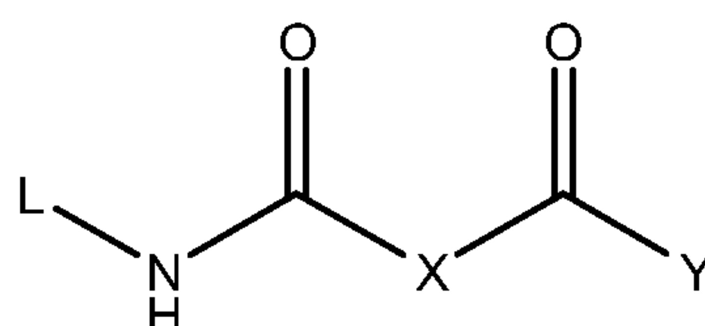
Formula (I)
