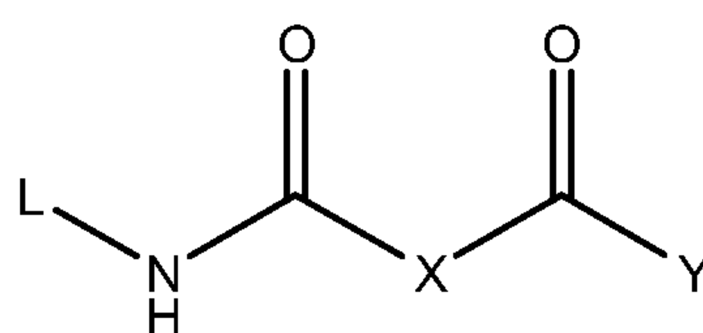
Formula (I)
