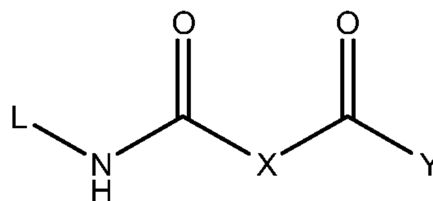
Formula (II)
