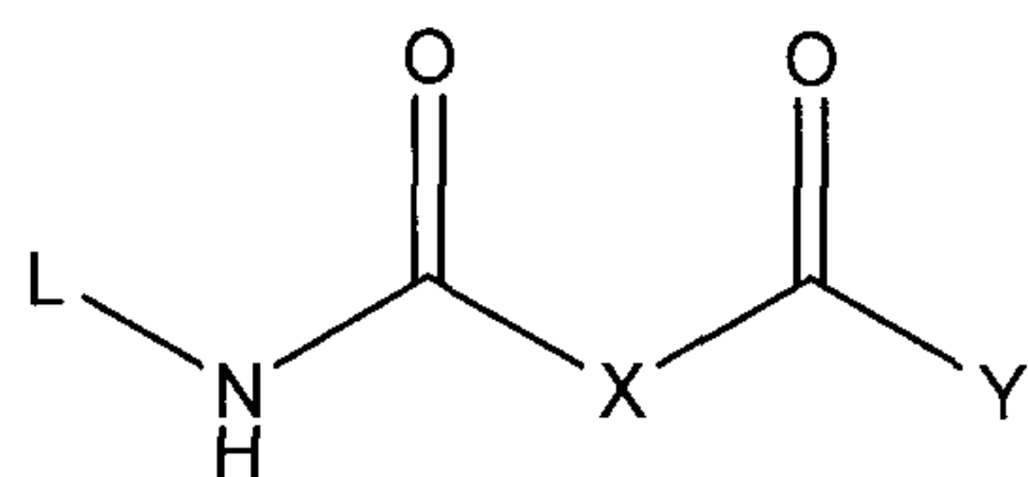
Formula (I)
