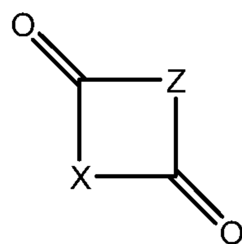
Formula (III)
