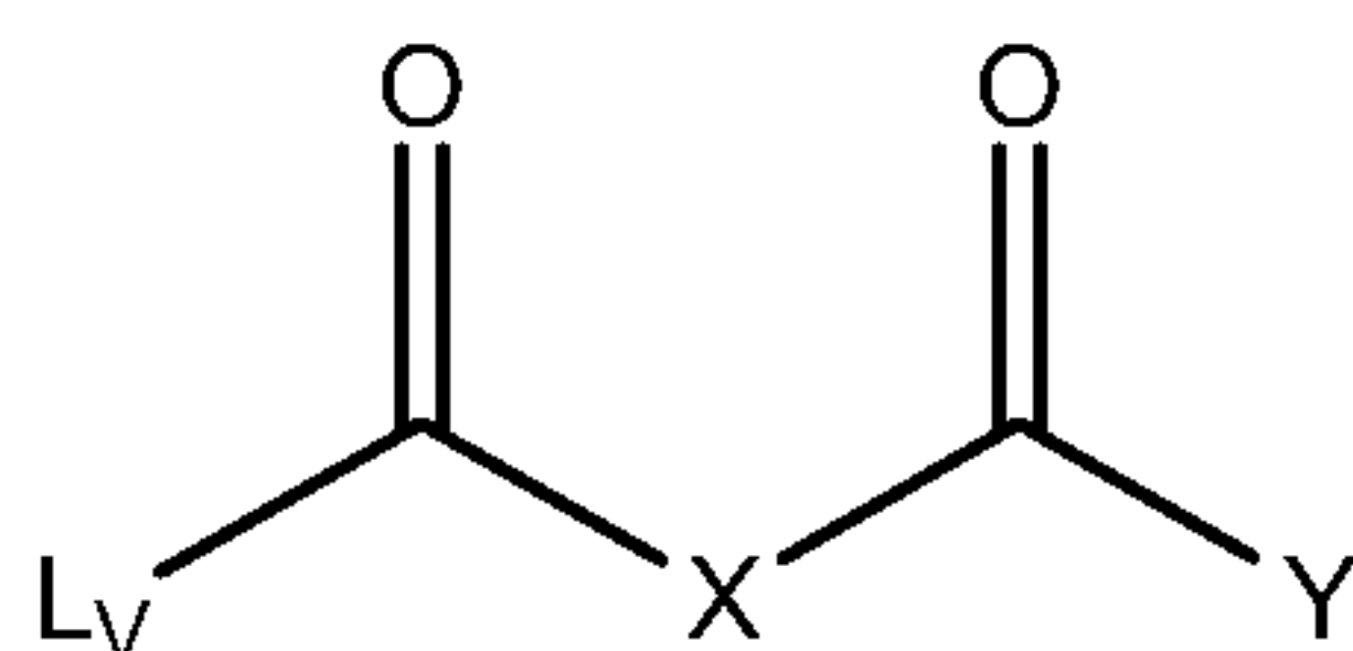
Formula (IV)
