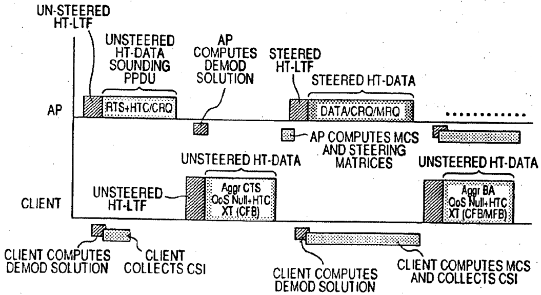
FIG. 12 PRIOR ART
