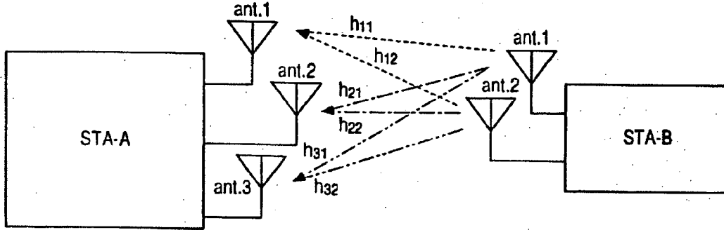
FIG. 11 PRIOR ART
