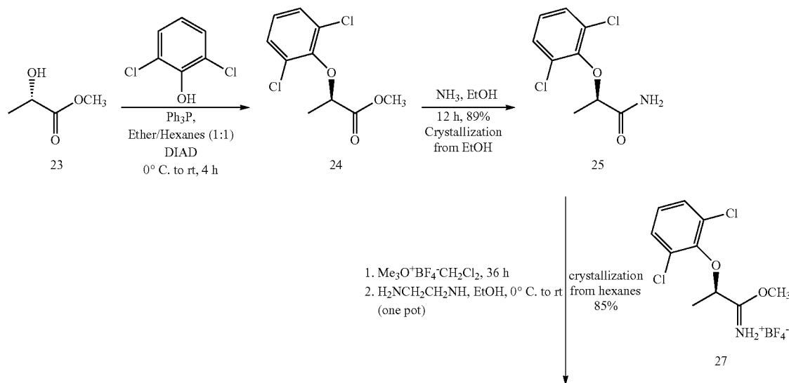
Scheme 4. Synthesis of (−)-lofexidine (3).
