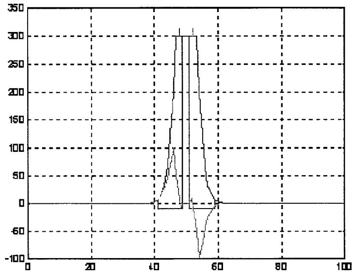
Figure 33: Twin towers detected (where only one exists.)
