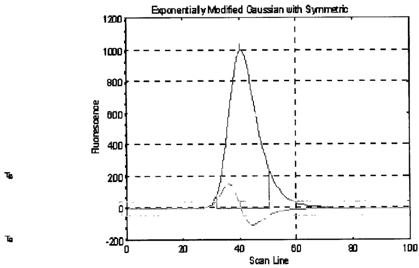
Figure 27: Do not set symmetric parameters if the peak is not symmetric.
