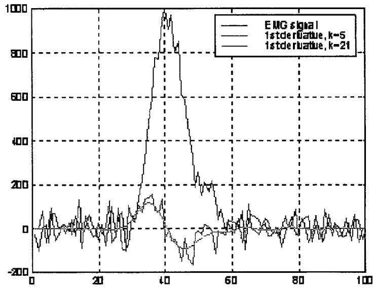
Figure 31: Using k to smooth the derivative.
