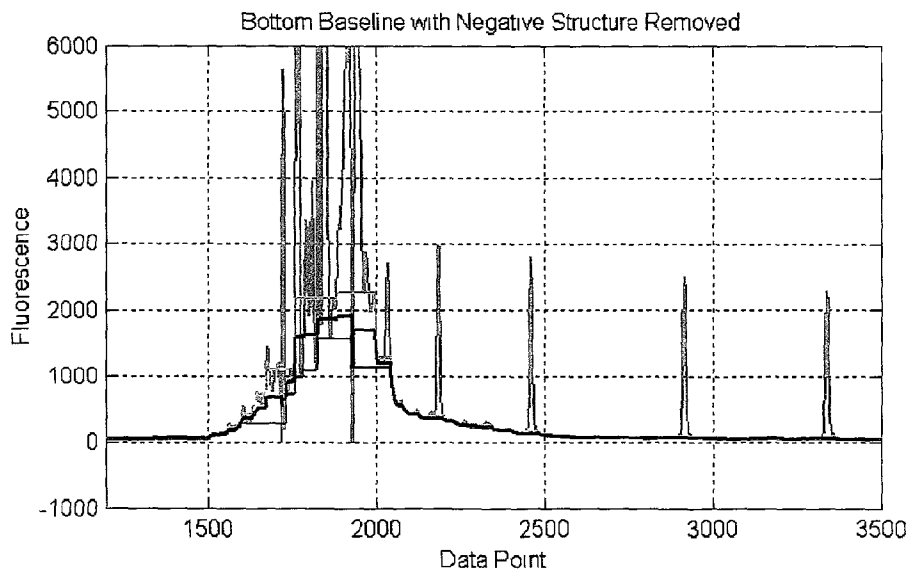
Figure 22: Baseline by averaging the top and bottom.
