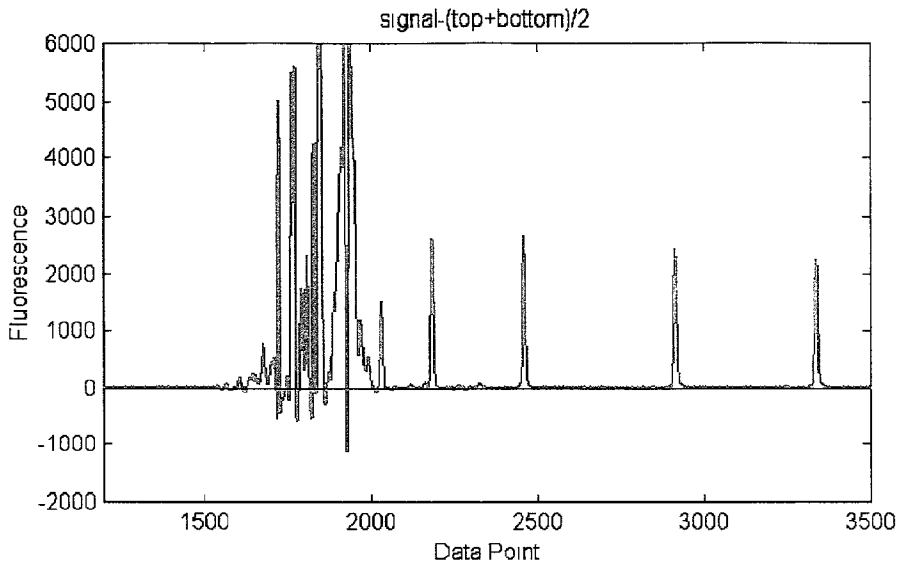
Figure 23: The baselined signal. Note negative values.
