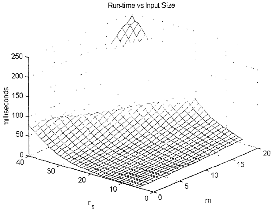
Figure 40: A mesh of execution times.
