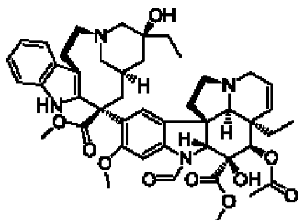
Vincristine
