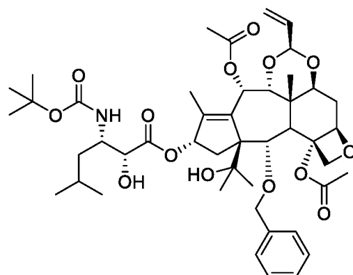
abeo-taxane15a.2
