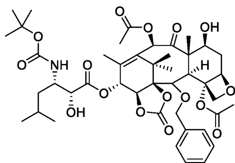
Orataxel
