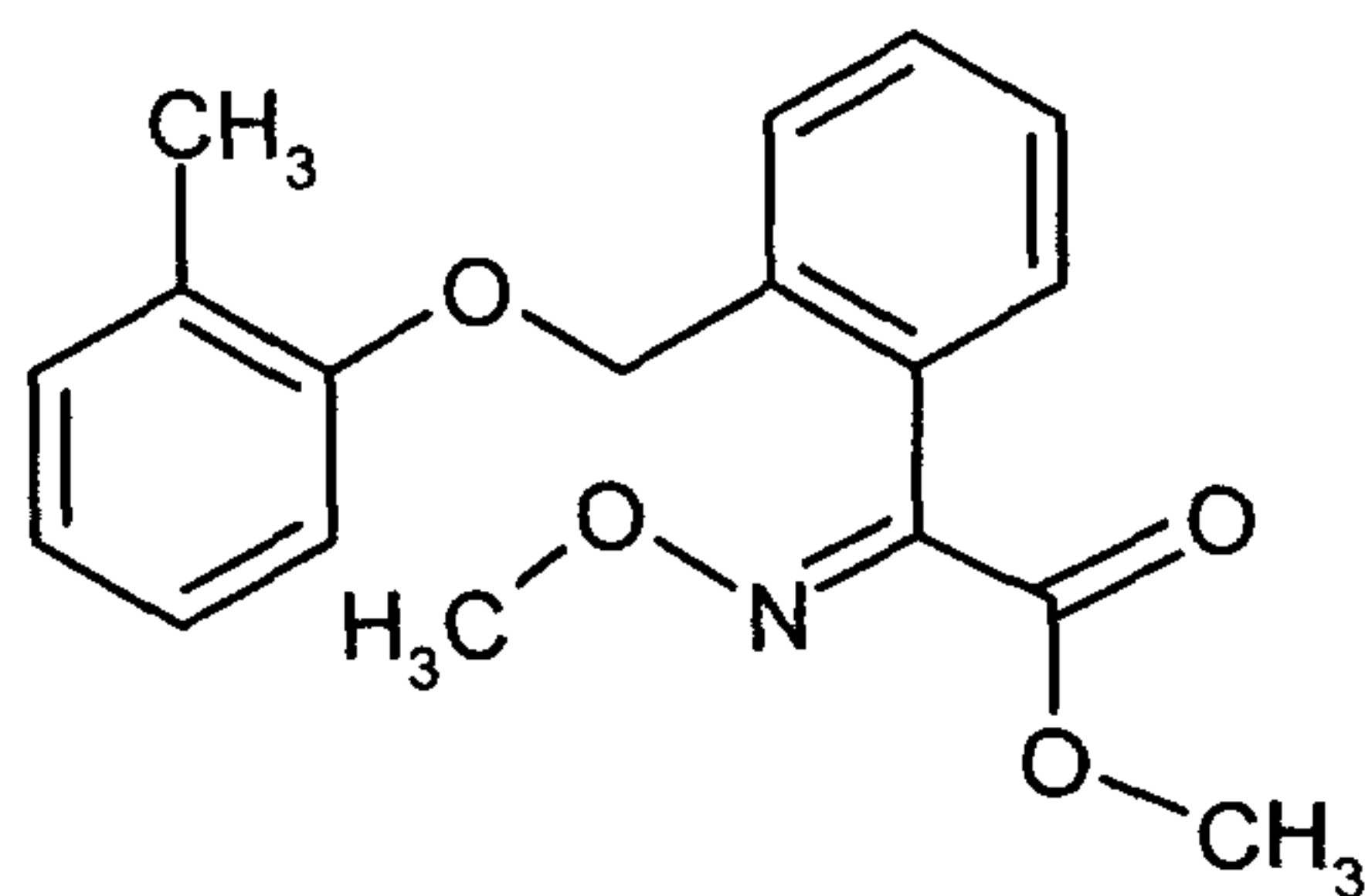
(Kresoxim-methyl)
