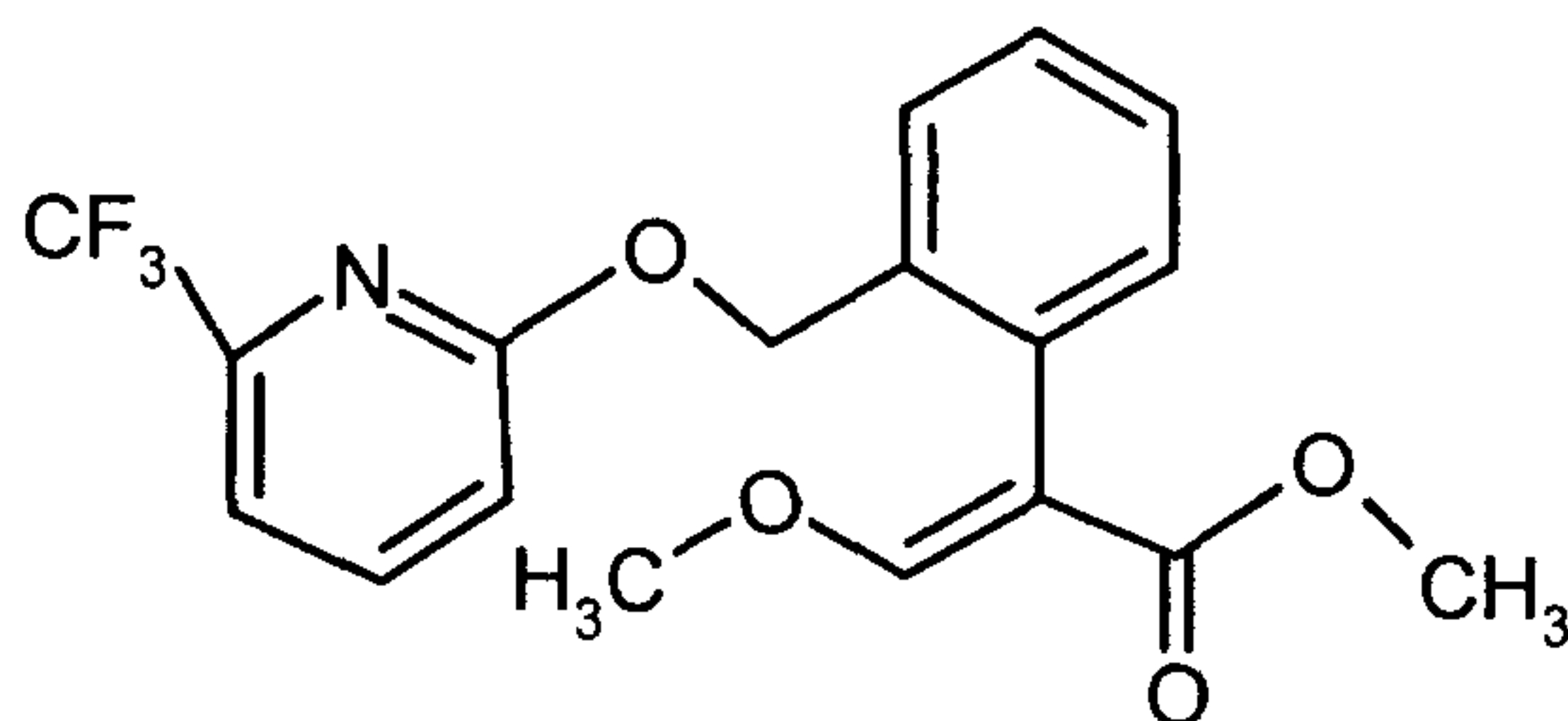
(Picoxystrobin)
