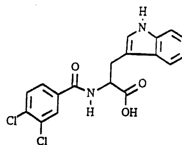
Figure: Some Representative CCK/Gastrin Receptor Ligands
