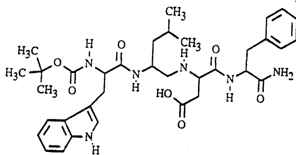
Figure: Some Representative CCK/Gastrin Receptor Ligands
