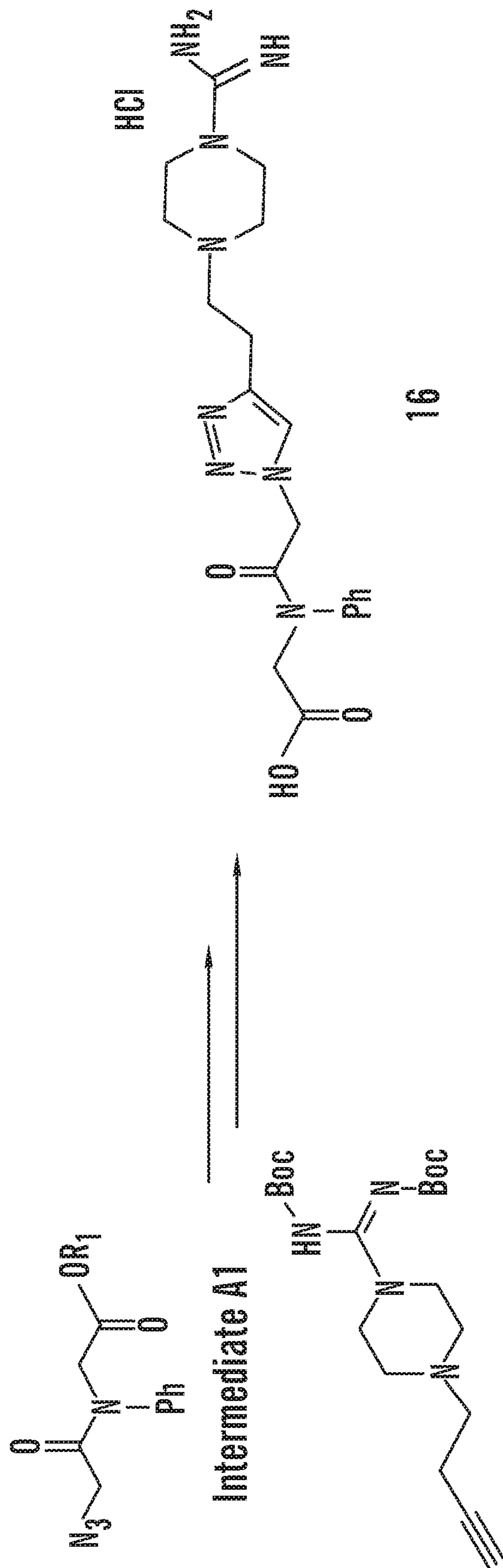
Scheme 4. General synthetic scheme of compound 16 [34].
