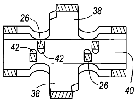
FIG. 3B SECTION A A
