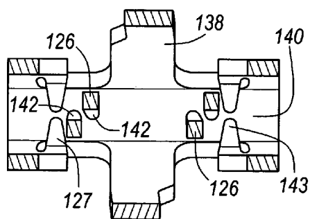
FIG. 14B SECTION A A
