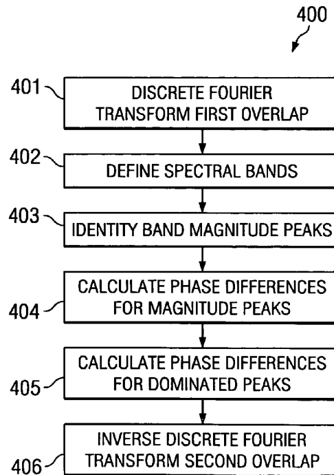
FIG. 4 (PRIOR ART)
