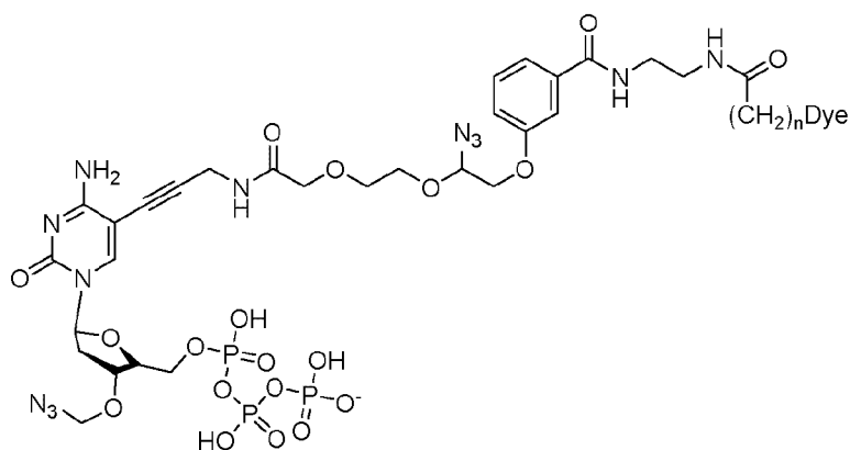
ffC-LN3-Dye
