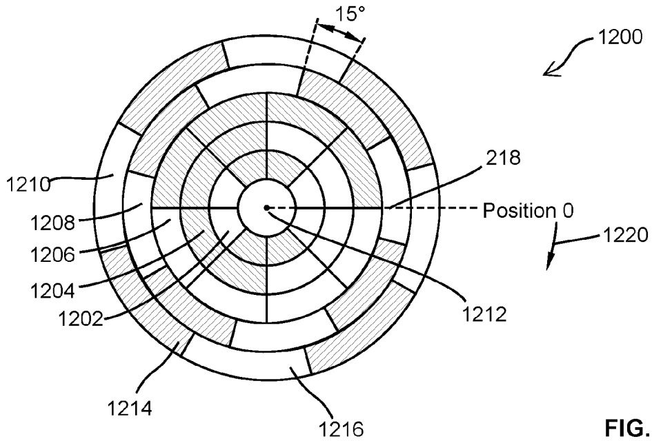
Encoder with 2 Booster Channels
