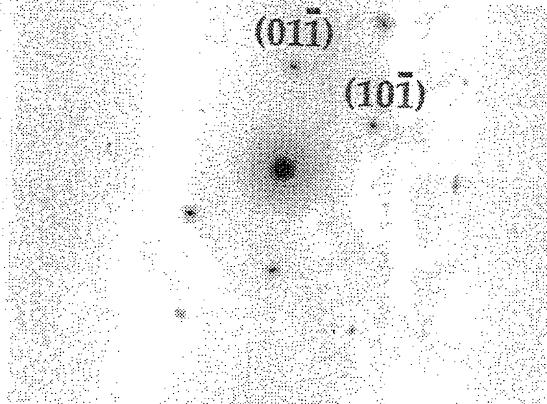
SAD Pattern Corresponding to [111] zone axis of alumina
