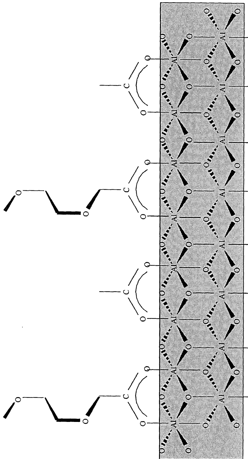
Mixed-Ligand Alumoxanes: MEA-A and A-A
