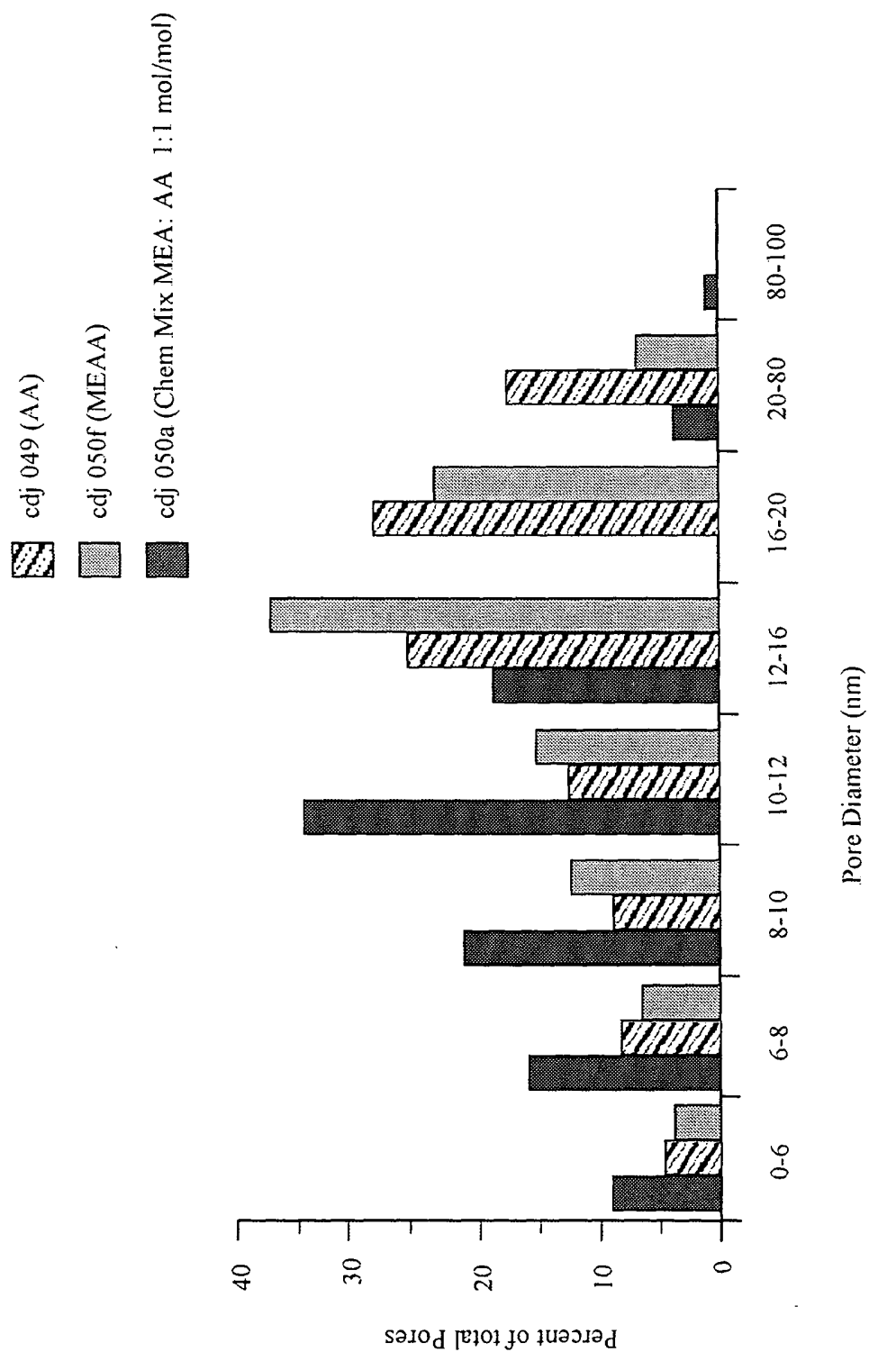
Comparisons of Pore Diameters for AA, MEAA and Chem MEA/AA
