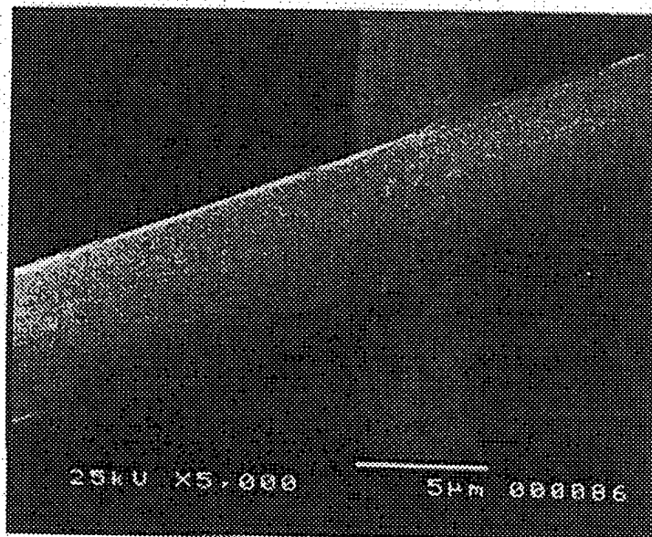
Akzo Fortafil 3C(unt) 7 \mu m carbon fibers, YAG coated
