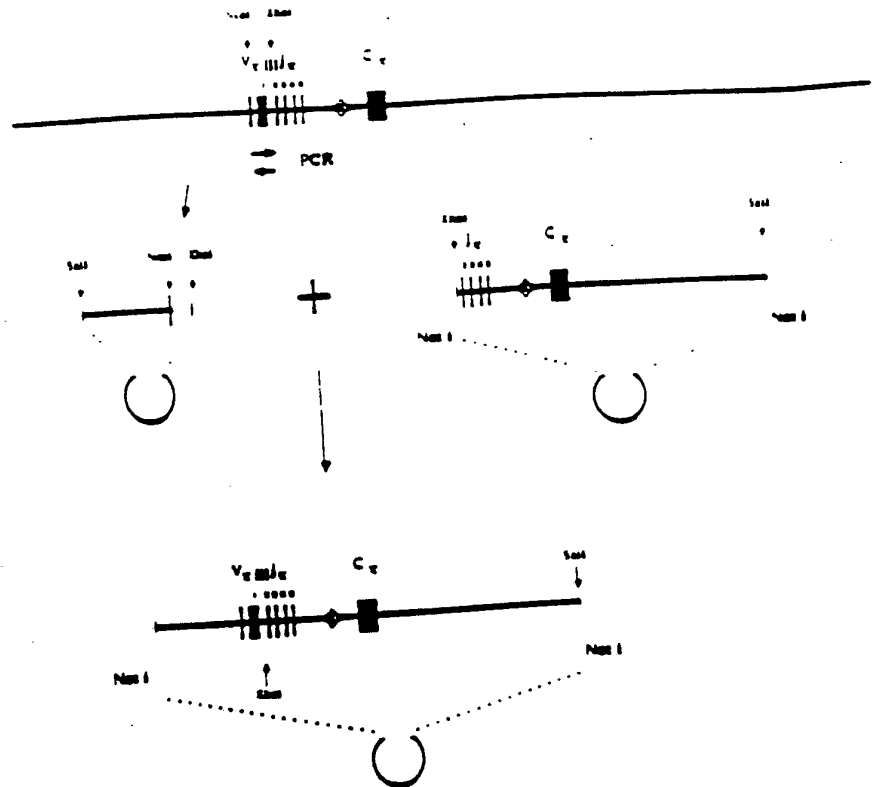
Expression cassette for rearranged \kappa light chain genes.
