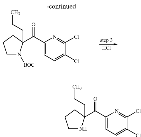
Step 1 2-[(5,6-Dichloro-pyridin-2-yl)-hydroxy-methyl]-2-propyl-pyrrolidine-1-carboxylic acid tert-butyl ester
