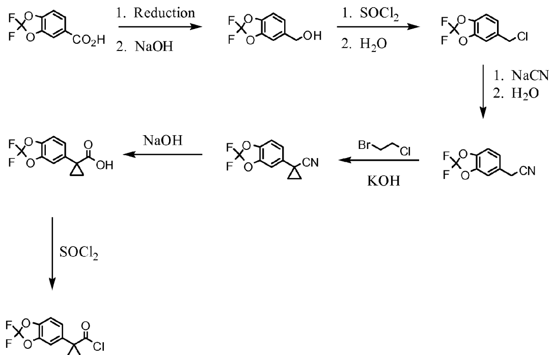
Scheme 3. Synthesis of the amine moiety.
