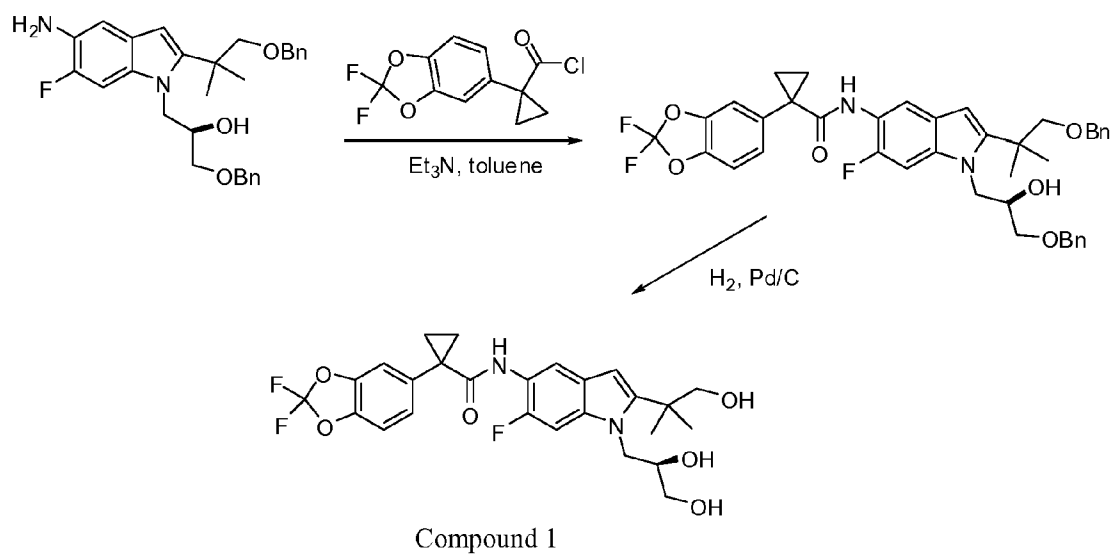
Scheme 4. Formation of Compound 1.
