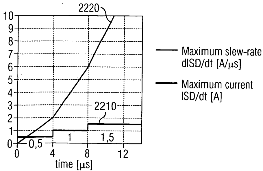
FIG 18 PRIOR ART
