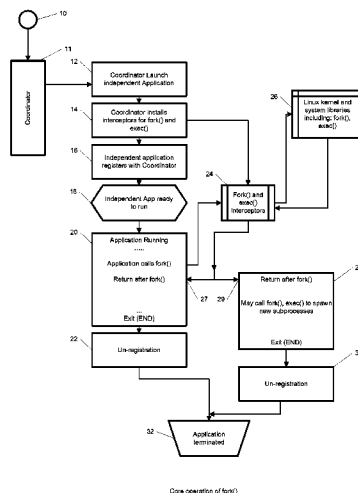
Core operation of fork()
