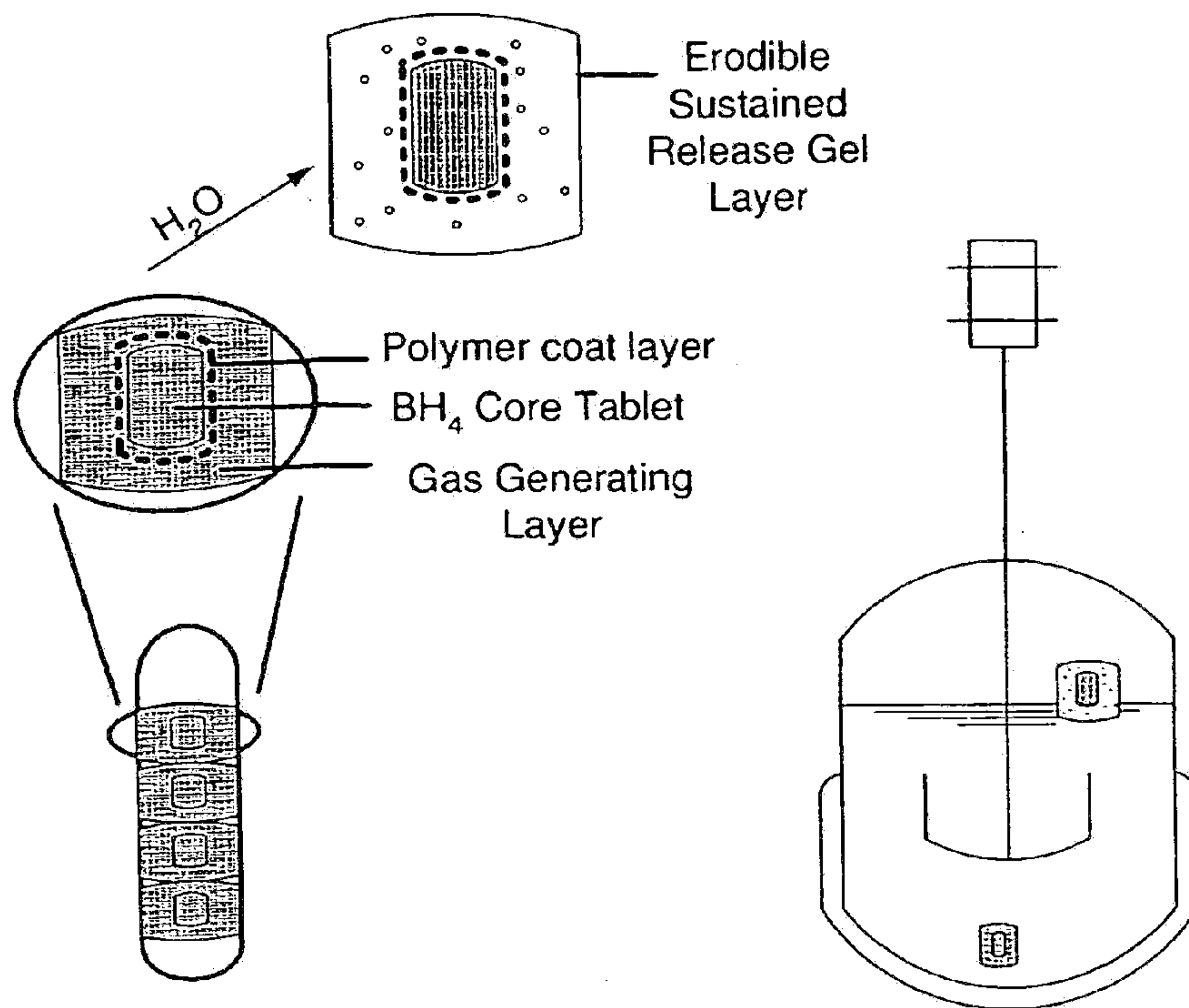
FIGURE 34 Schematic Diagram of Gas Generating Dosage Form
