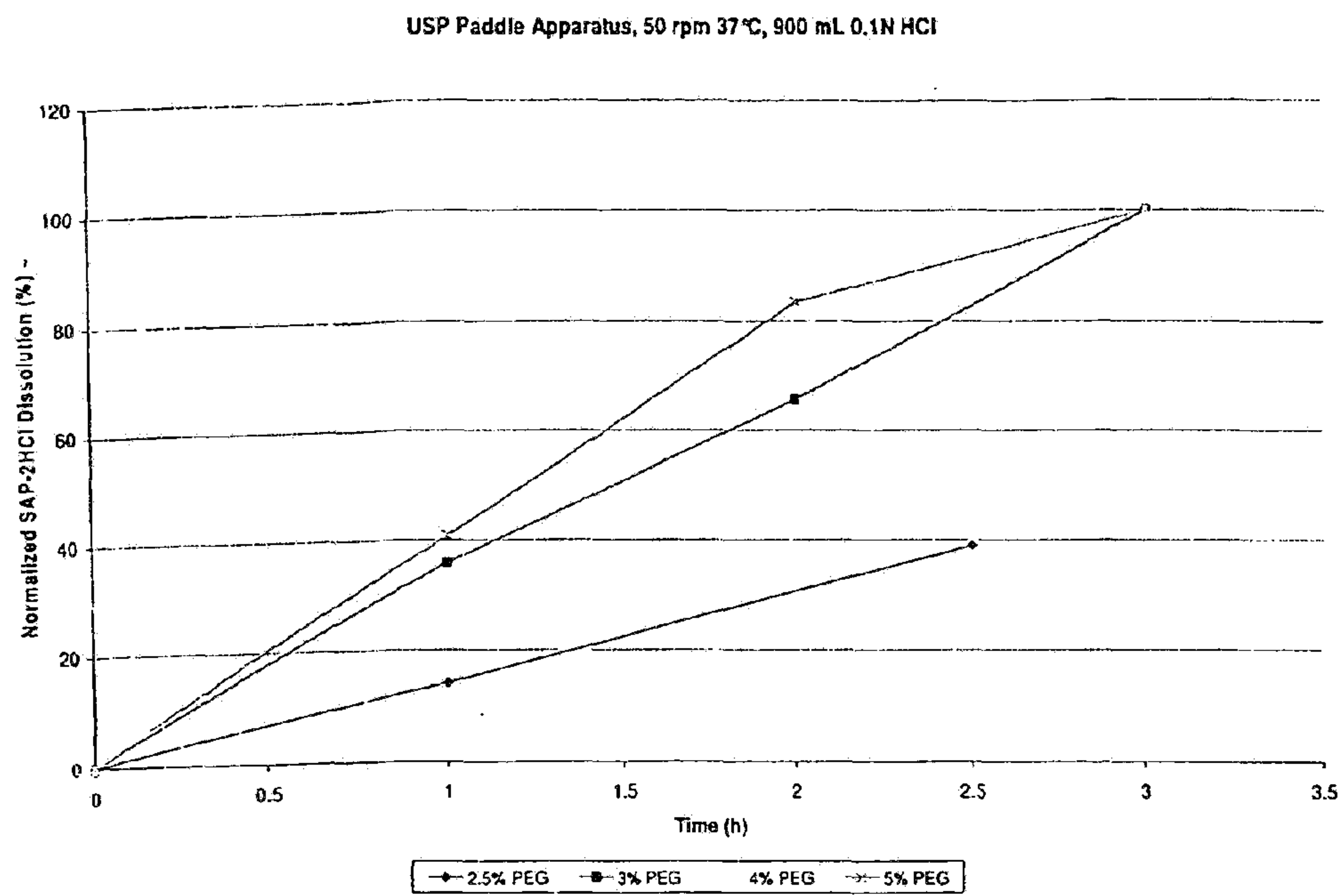
FIGURE 33 Dissolution Profile of Floating System Prototype (80 mg BH4) with Varying Levels of PEG Coating
