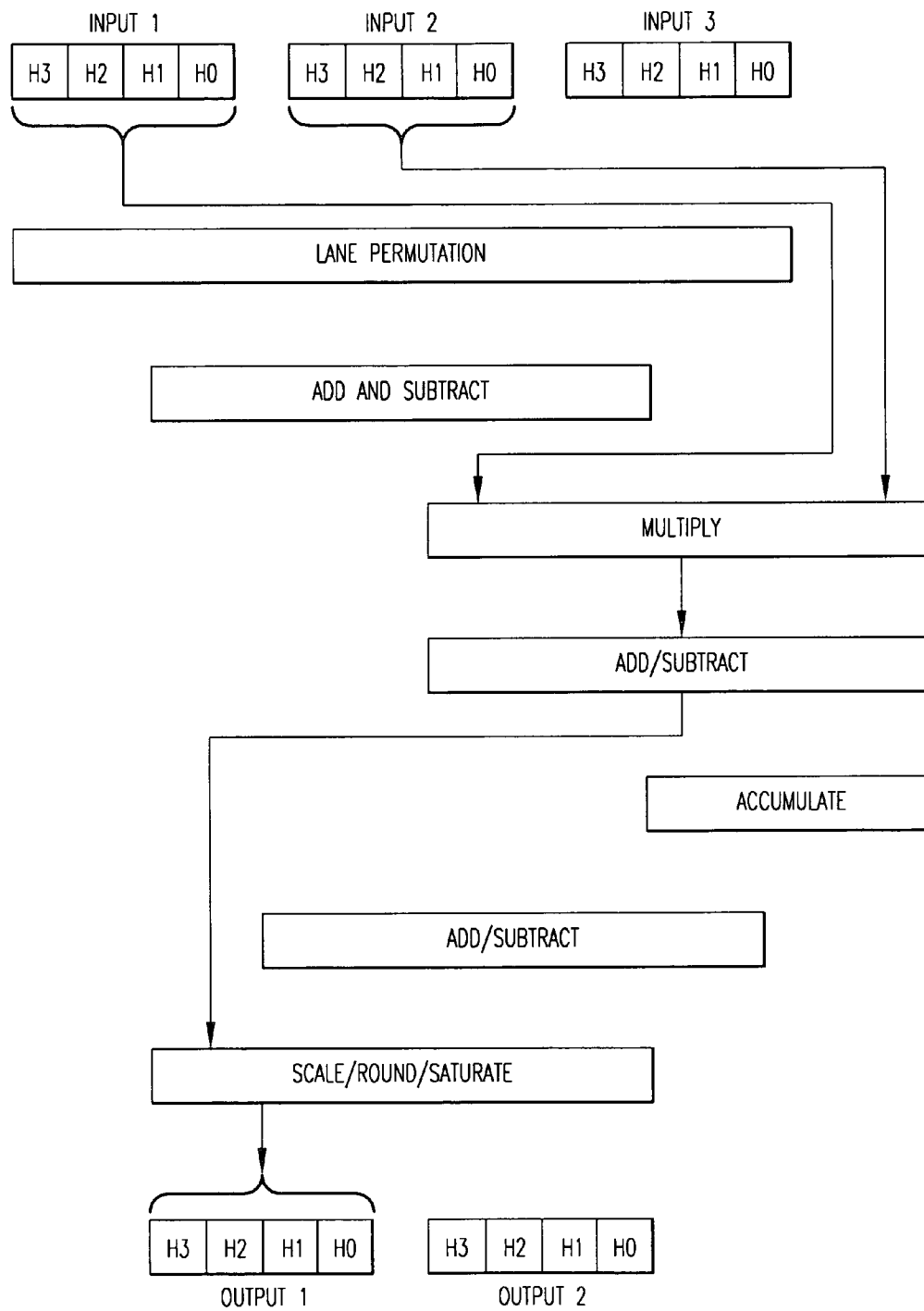
CMULH DATA FLOW
