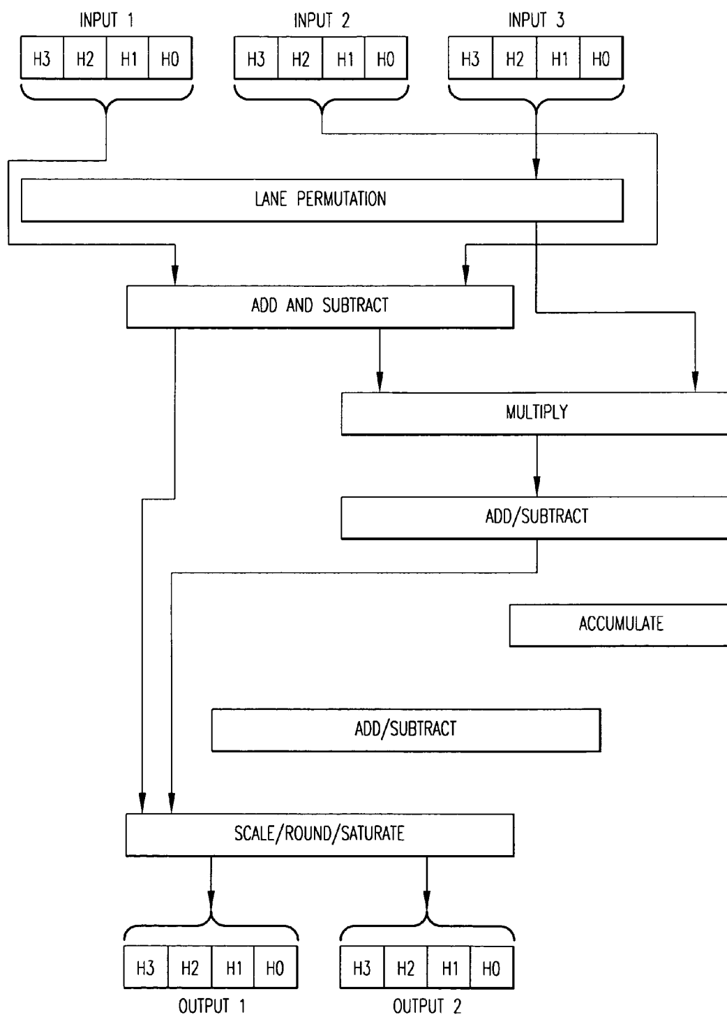
BFLYH DATA PROCESSING FLOW
