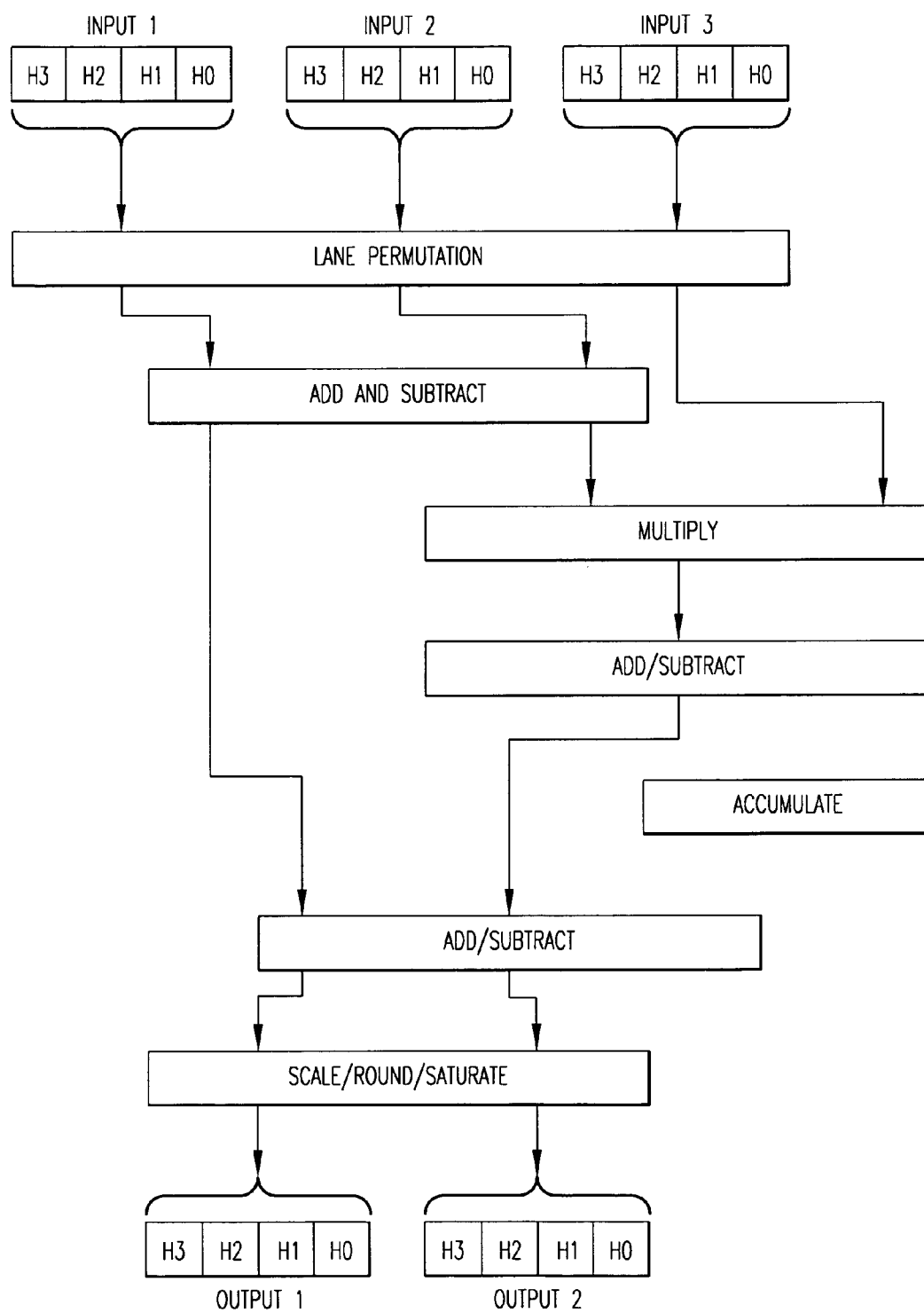
BFLYH-CVT DATA PROCESSING FLOW
