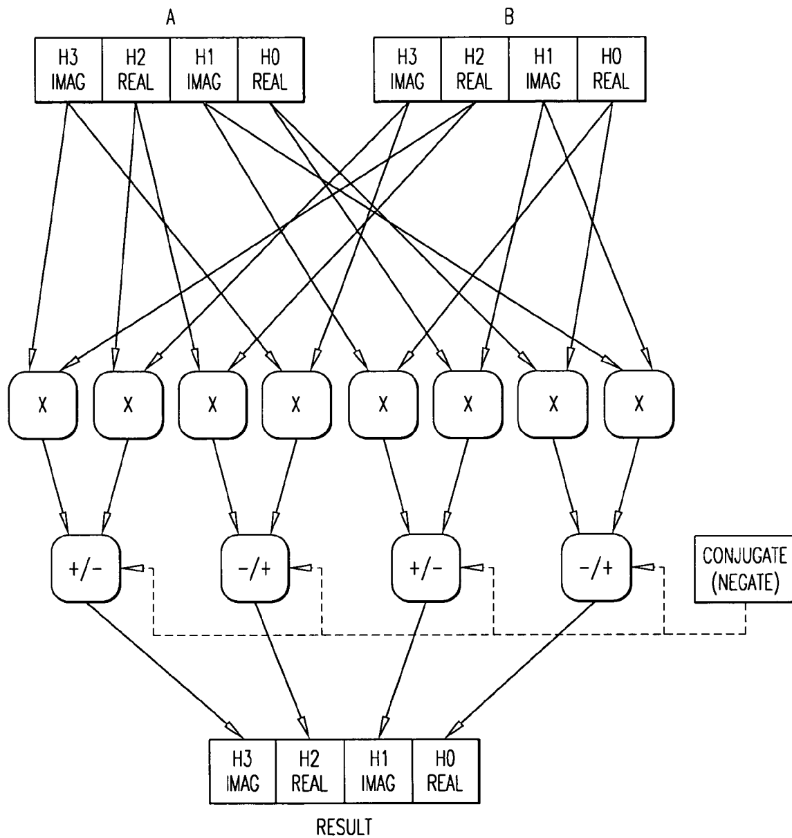
MULTIPLY AND ADD/SUBTRACT BLOCK DETAIL FOR CMULH
