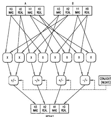
MULTIPLY AND ADD/SUBTRACT BLOCK DETAIL FOR CMULH
