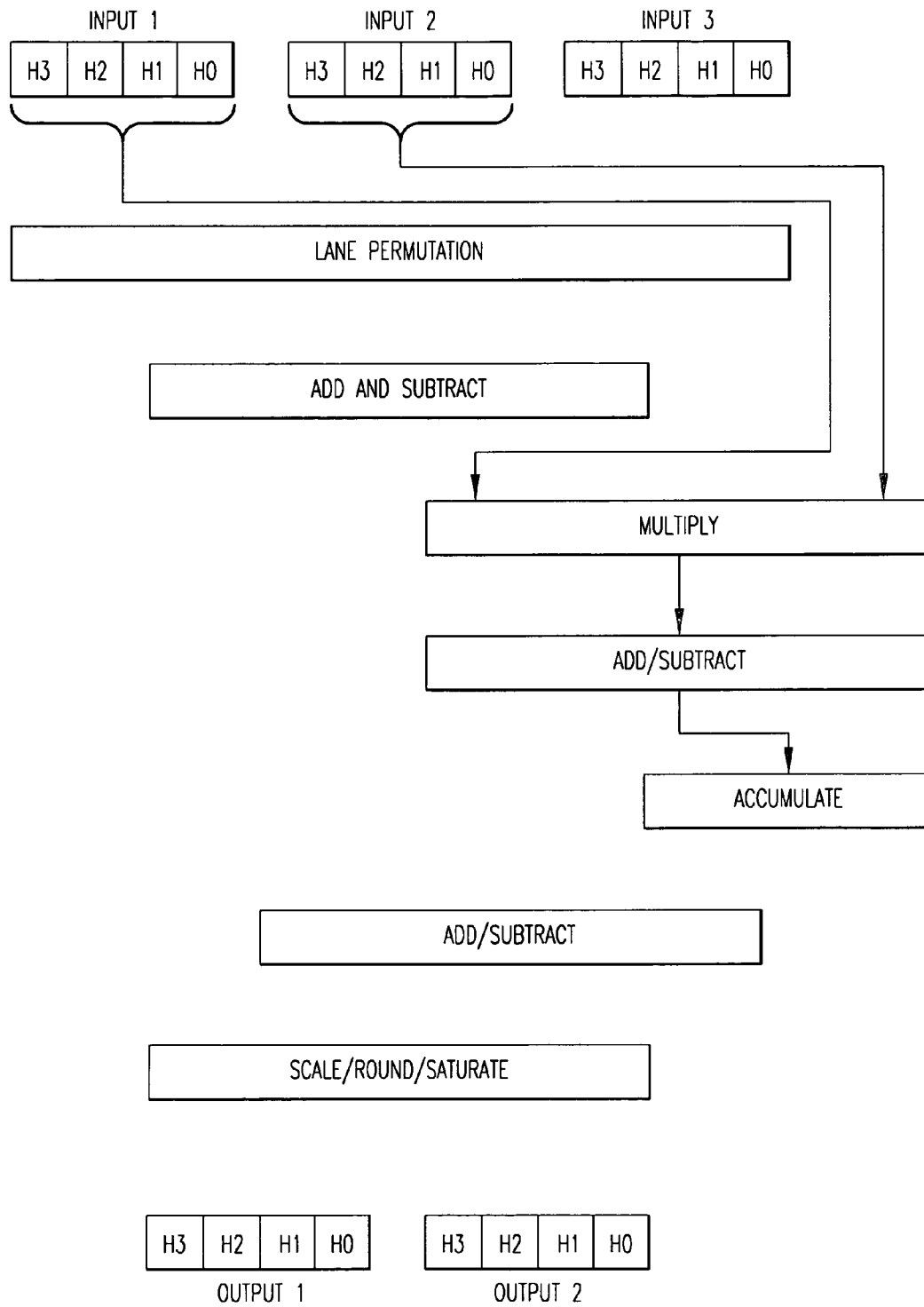
CMACH DATA PROCESSING FLOW
