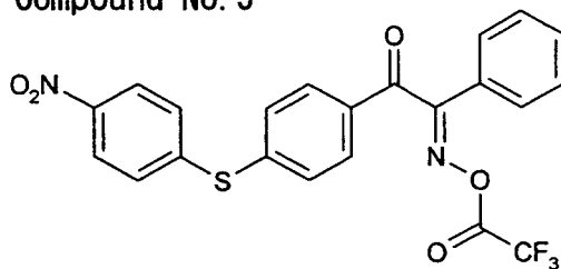
Compound No. 5
