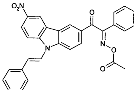
Compound No. 23
