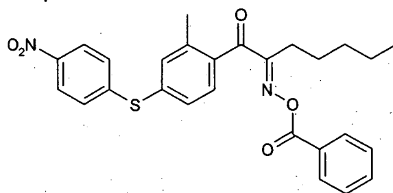
Compound No. 10
