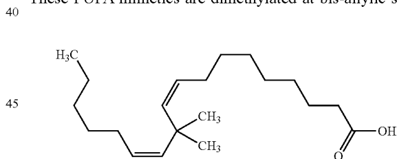
11,11-Dimethyl-octadeca-9,12-dienoic acid
