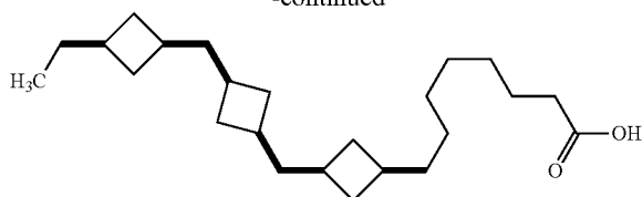
8-(3-[3-(3-Ethyl-cyclobutylmethyl)-cyclobutylmethyl]-cyclobutyl-octanoic acid
