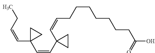
10-{1-[2-(1-But-1-enyl-cyclopropyl)-vinyl]-cyclopropyl}-dec-9-enoic acid
