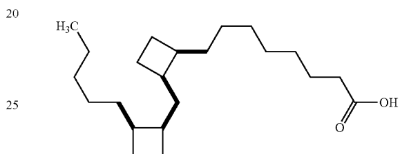
8-[2-(2-Pentyl-cyclobutylmethyl)-cyclobutyl]-octanoic acid
