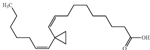
10-(1-Hept-1-enyl-cyclopropyl)-dec-9-enoic acid
