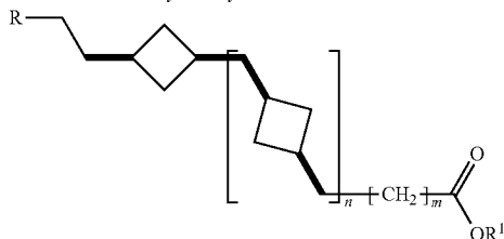
8-(3-[3-(3-Ethyl-cyclobutylmethyl)-cyclobutylmethyl]-cyclobutyl-octanoic acid
