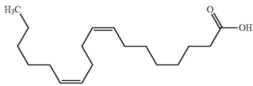
Octadeca-8,12-dienoic acid
