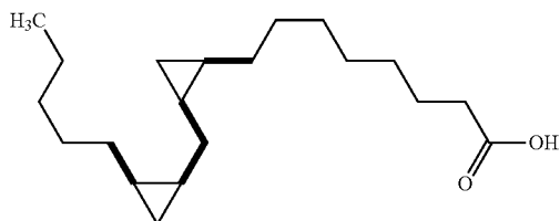
8-[2-(2-Pentyl-cyclopropylmethyl)-cyclopropyl]-octanoic acid
