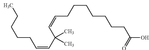
11,11-Dimethyl-octadeca-9,12-dienoic acid
