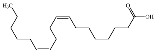
Octadeca-8,12-dienoic acid
