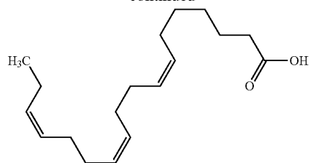
Octadeca-7,11,15-trienoic acid
