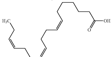
Octadeca-7,11,15-trienoic acid
