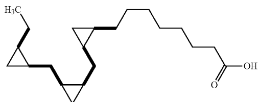
8-{2-[2-(2-Ethyl-cyclopropylmethyl)-cyclopropylmethyl]-cyclopropyl}-octanoic acid
