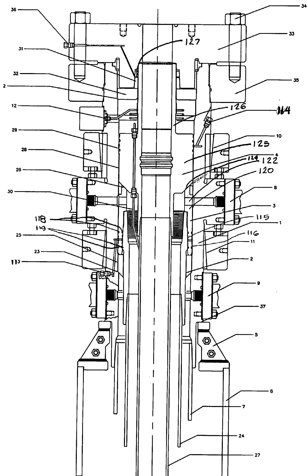
FIGURE 2 "HG" WELLHEAD CONFIGURATION 1
