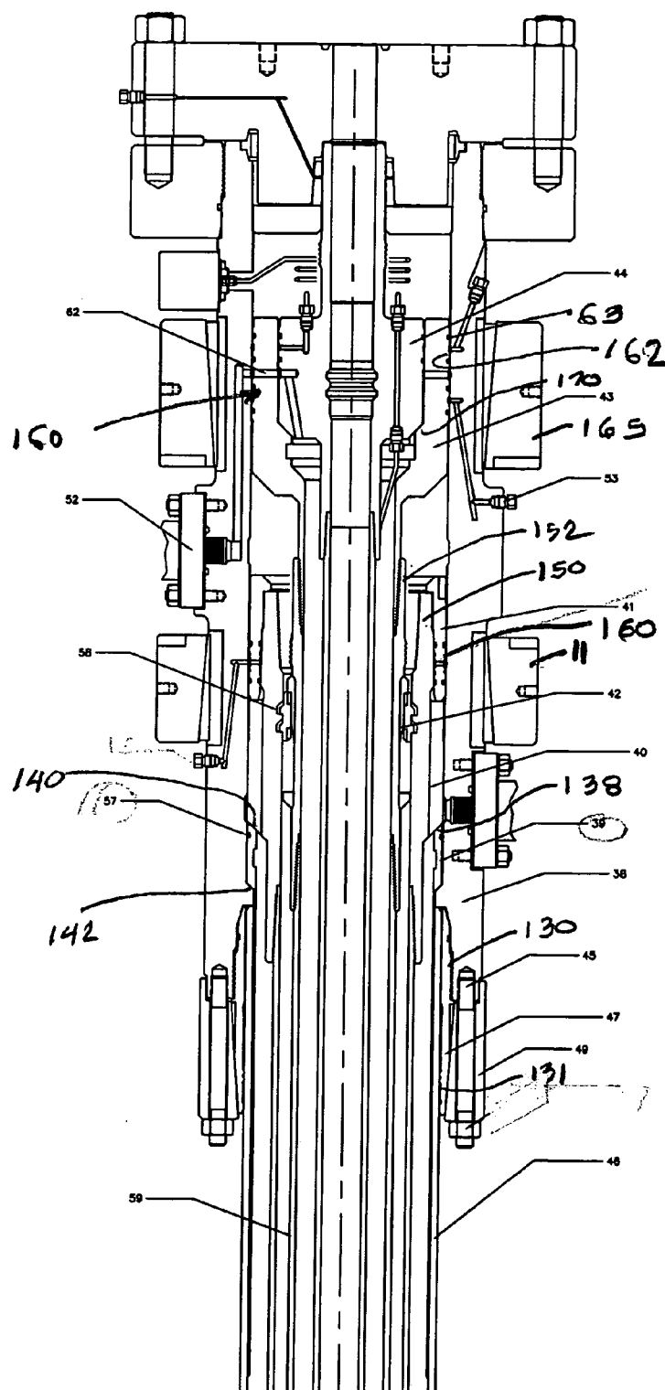
FIGURE 4: "HG" WELLHEAD CONFIGURATION 2 SECTION A-A
