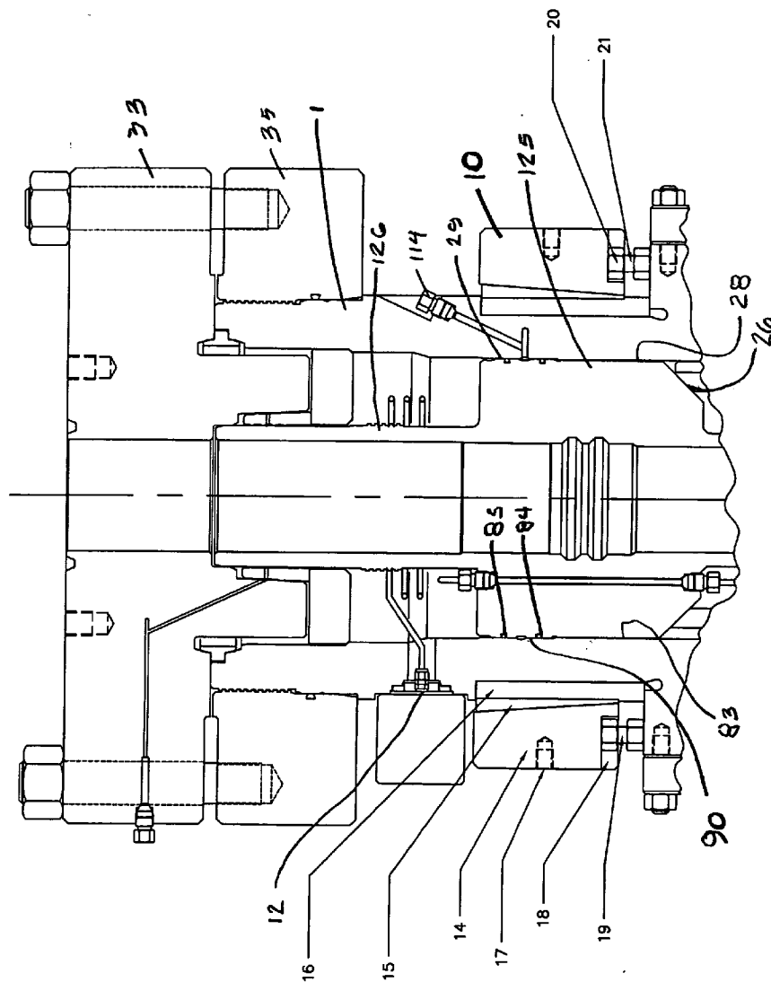
FIGURE 3: "HC" WELLHEAD CONFIGURATION 1 TUBING HANGER & POS-GRIP DETAIL
