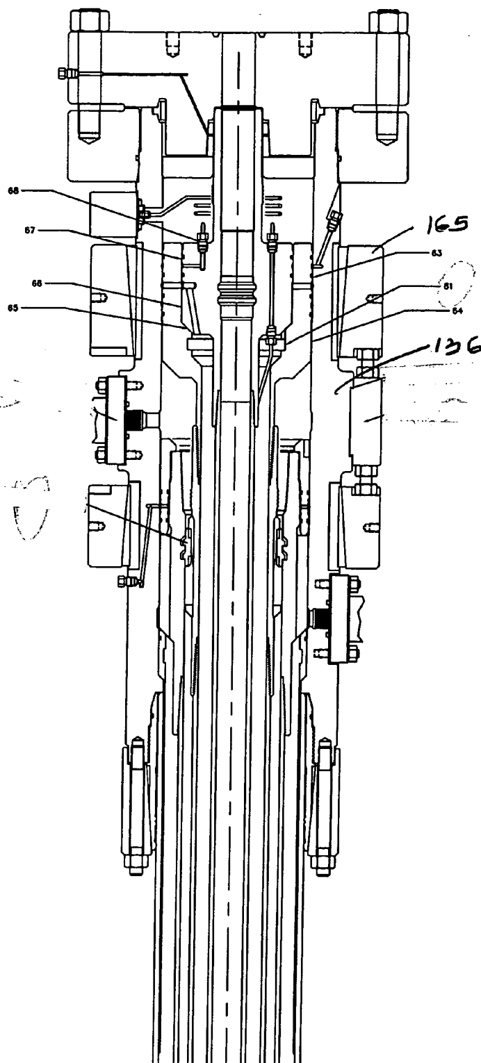
FIGURE 5 "HG" WELLHEAD CONFIGURATION 2 SECTION B-B
